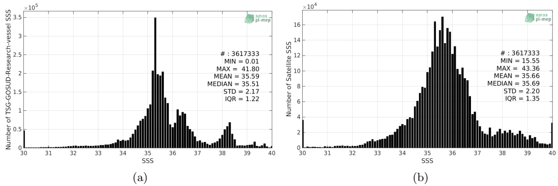
Figure 2: Histograms of SSS from TSG-GOSUD-Research-vessel (a) and SMOS-L3-CATDS-CECOS-LOCEAN-V4-9DAYS-25KM (b) considering all match-up pairs per bins of 0.1 over the SMOS coastal zone ( \geq 800 km) 60N-60S Pi-MEP region and for the full satellite product period.
