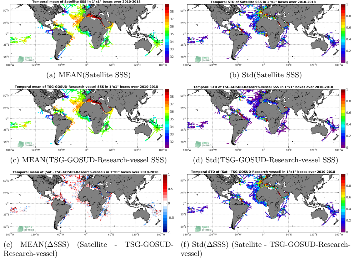
Figure 6: Temporal mean (left) and Std (right) of SSS from SMOS-L3-CATDS-CECOS-LOCEAN-V4-9DAYS-25KM (top), TSG-GOSUD-Research-vessel (middle), and of \Delta SSS (Satellite - TSG-GOSUD-Research-vessel). Only match-up pairs are used to generate these maps.
