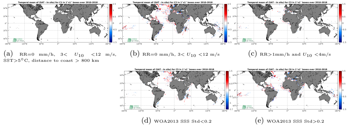
Figure 12: Temporal mean gridded over spatial boxes of size 1^\circ \times 1^\circ of \Delta SSS (SMOS-L3-CATDS-CECOS-LOCEAN-V4-9DAYS-25KM - TSG-GOSUD-Research-vessel) for 5 different subdatasets corresponding to:RR=0 mm/h, 3 < U_{10} < 12 m/s, SST >5^\circ\text{C} , distance to coast > 800 km (a), RR=0 mm/h, 3 < U_{10} < 12 m/s (b), RR >1 mm/h and U_{10} < 4 m/s (c), WOA2013 SSS Std <0.2 (d), WOA2013 SSS Std >0.2 (e).
