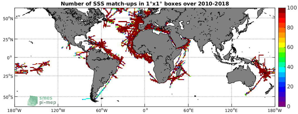
Figure 4: Number of SSS match-ups between TSG-GOSUD-Research-vessel SSS and the SMOS-L3-CATDS-CECOS-LOCEAN-V4-9DAYS-25KM SSS product for the SMOS coastal zone ( \geq 800\text{km} ) 60N-60S Pi-MEP region over 1^\circ \times 1^\circ boxes and for the full satellite product period.
