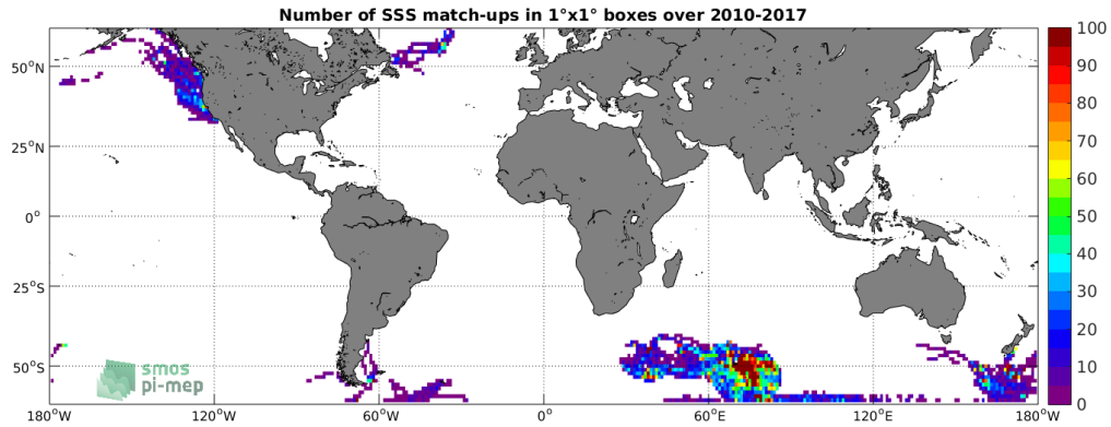
Figure 4: Number of SSS match-ups between Sea mammals SSS and the SMOS-L3-CATDS-CECOS-LOCEAN-V4-9DAYS-25KM SSS product for the SMOS coastal zone (<800km) 60N-60S Pi-MEP region over 1°x1° boxes and for the full satellite product period.
