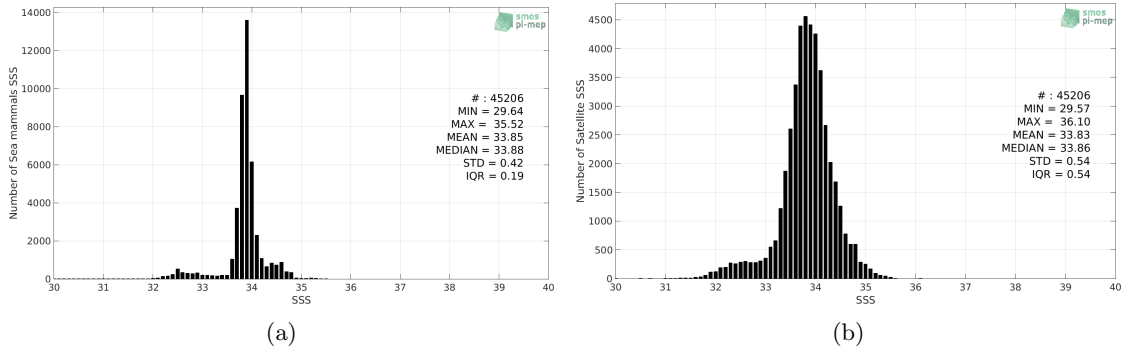
Figure 2: Histograms of SSS from Sea mammals (a) and SMOS-L3-CATDS-CECOS-LOCEAN-V4-9DAYS-25KM (b) considering all match-up pairs per bins of 0.1 over the SMOS coastal zone (<800km) 60N-60S Pi-MEP region and for the full satellite product period.
