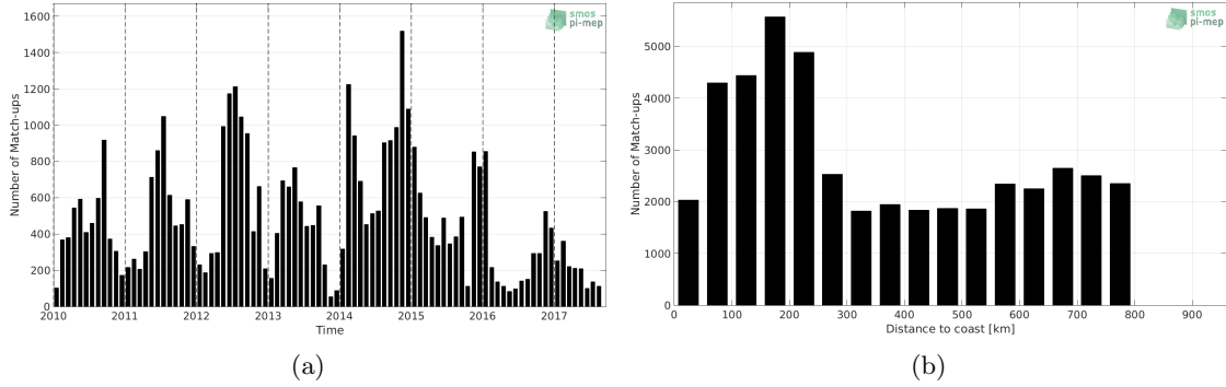
Figure 1: Number of match-ups between Sea mammals and SMOS-L3-CATDS-CECOS-LOCEAN-V4-9DAYS-25KM SSS as a function of time (a) and as function of the distance to coast (b) over the SMOS coastal zone (<800km) 60N-60S Pi-MEP region and for the full satellite product period.
