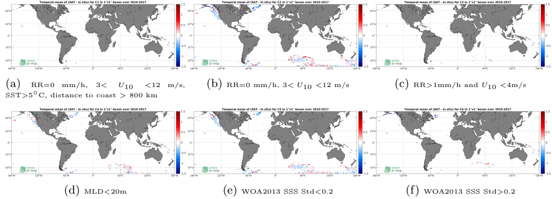
Figure 12: Temporal mean gridded over spatial boxes of size 1^{\circ}\times 1^{\circ} of \Delta\text{SSS} (SMOS-L3-CATDS-CECOS-LOCEAN-V4-9DAYS-25KM - Sea mammals) for 6 different subdatasets corresponding to: \text{RR}=0 mm/h, 3 < U_{10} < 12 m/s, \text{SST} > 5^{\circ}\text{C} , distance to coast > 800 km (a), \text{RR}=0 mm/h, 3 < U_{10} < 12 m/s (b), \text{RR} > 1\text{mm/h} and U_{10} < 4\text{m/s} (c), \text{MLD} < 20\text{m} (d), WOA2013 SSS Std < 0.2 (e), WOA2013 SSS Std > 0.2 (f).
