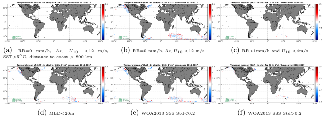
Figure 12: Temporal mean gridded over spatial boxes of size 1^\circ \times 1^\circ of \Delta SSS (SMOS-L3-CATDS-CECOS-LOCEAN-V4-9DAYS-25KM - Sea mammals) for 6 different subdatasets corresponding to: RR=0 mm/h, 3 < U_{10} < 12 m/s, SST > 5^\circ\text{C} , distance to coast > 800 km (a), RR=0 mm/h, 3 < U_{10} < 12 m/s (b), RR > 1 mm/h and U_{10} < 4 m/s (c), MLD < 20 m (d), WOA2013 SSS Std < 0.2 (e), WOA2013 SSS Std > 0.2 (f).
