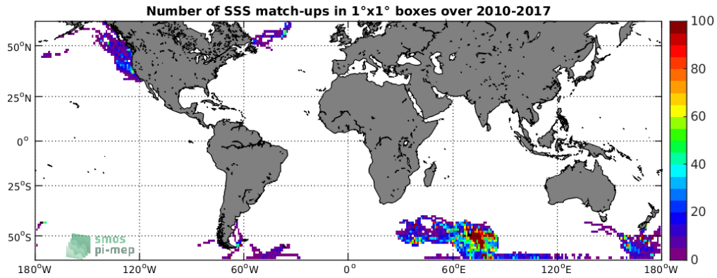
Figure 4: Number of SSS match-ups between Sea mammals SSS and the SMOS-L3-CATDS-CECOS-LOCEAN-V4-9DAYS-25KM SSS product for the SMOS coastal zone ( \geq 800\text{km} ) 60^\circ\text{N} - 60^\circ\text{S} Pi-MEP region over 1^\circ \times 1^\circ boxes and for the full satellite product period.
