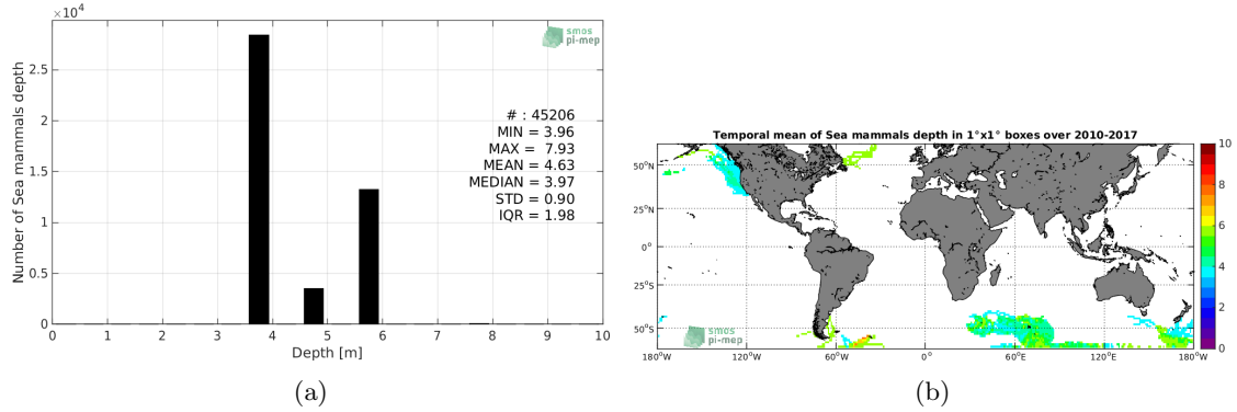
Figure 3: Histograms of the depth of the upper level SSS measurements from Sea mammals in the Match-up DataBase for the SMOS coastal zone ( \geq 800\text{km} ) 60^\circ\text{N} - 60^\circ\text{S} Pi-MEP region (a) and temporal mean spatial distribution of pressure of the in situ SSS data over 1^\circ \times 1^\circ boxes and for the full satellite product period (b).
