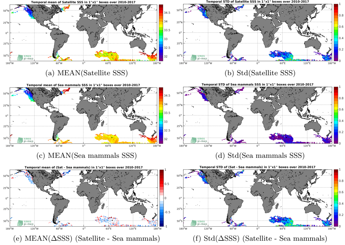
Figure 6: Temporal mean (left) and Std (right) of SSS from SMOS-L3-CATDS-CECOS-LOCEAN-V4-9DAYS-25KM (top), Sea mammals (middle), and of \Delta SSS (Satellite - Sea mammals). Only match-up pairs are used to generate these maps.
