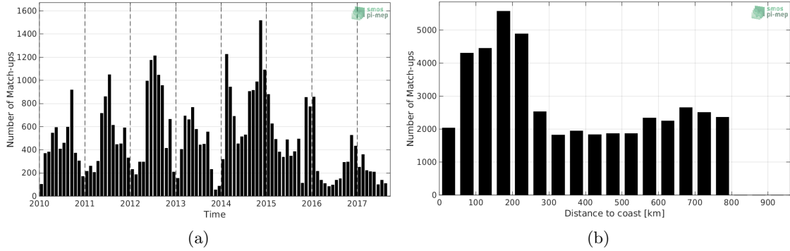
Figure 1: Number of match-ups between Sea mammals and SMOS-L3-CATDS-CECOS-LOCEAN-V4-9DAYS-25KM SSS as a function of time (a) and as function of the distance to coast (b) over the SMOS coastal zone ( \leq 800 km) 60N-60S Pi-MEP region and for the full satellite product period.
