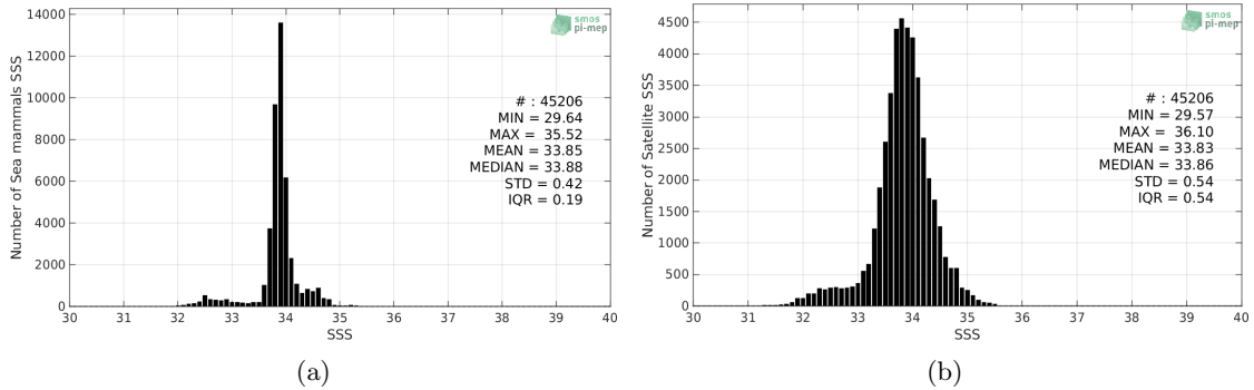
Figure 2: Histograms of SSS from Sea mammals (a) and SMOS-L3-CATDS-CECOS-LOCEAN-V4-9DAYS-25KM (b) considering all match-up pairs per bins of 0.1 over the SMOS coastal zone ( \leq 800 km) 60N-60S Pi-MEP region and for the full satellite product period.
