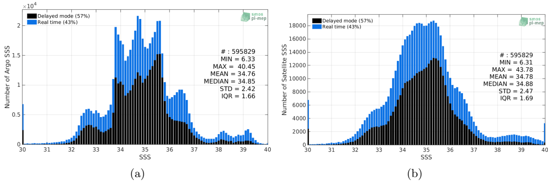
Figure 2: Histograms of SSS from Argo (a) and SMOS-L3-CATDS-CECOS-LOCEAN-V4-9DAYS-25KM (b) considering all match-up pairs per bins of 0.1 over the SMOS coastal zone ( \leq 800 km) 60N-60S Pi-MEP region and for the full satellite product period.
