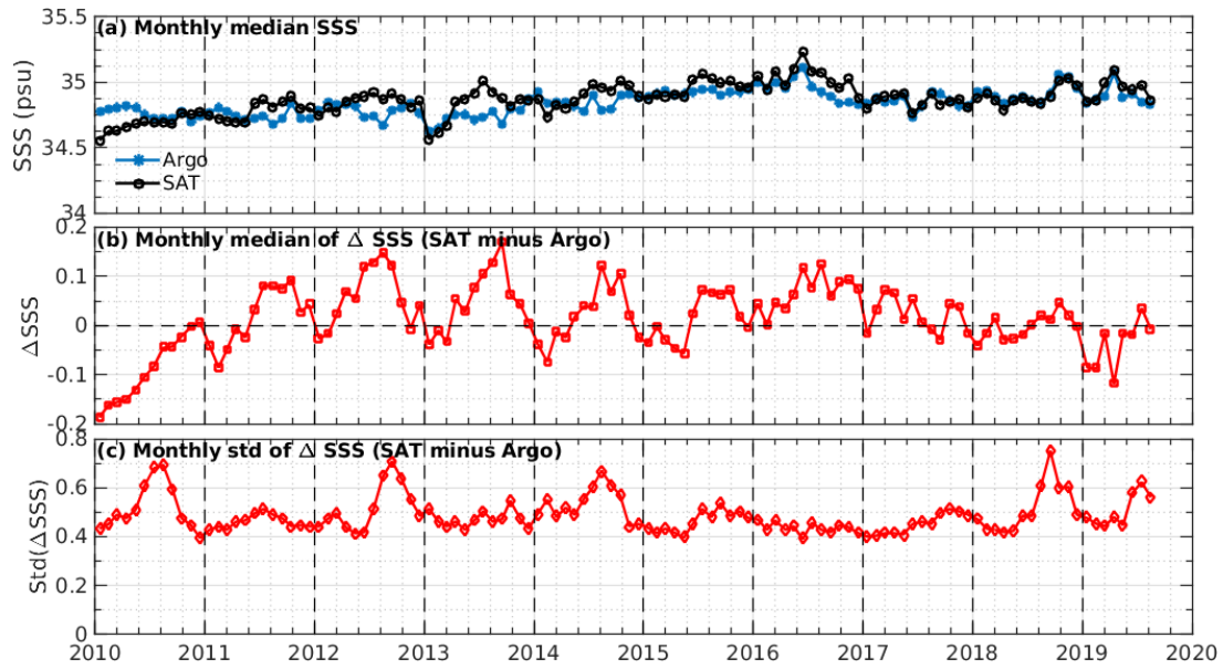
Figure 7: Time series of the monthly median SSS (top), median of \Delta SSS (Satellite - Argo) and Std of \Delta SSS (Satellite - Argo) over the SMOS coastal zone ( \approx 800 km) 60N-60S Pi-MEP region considering all match-ups collected by the Pi-MEP.
