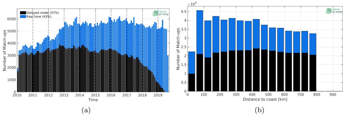
Figure 1: Number of match-ups between Argo and SMOS-L3-CATDS-CECOS-LOCEAN-V4-9DAYS-25KM SSS as a function of time (a) and as function of the distance to coast (b) over the SMOS coastal zone ( \leq 800 km) 60N-60S Pi-MEP region and for the full satellite product period.
