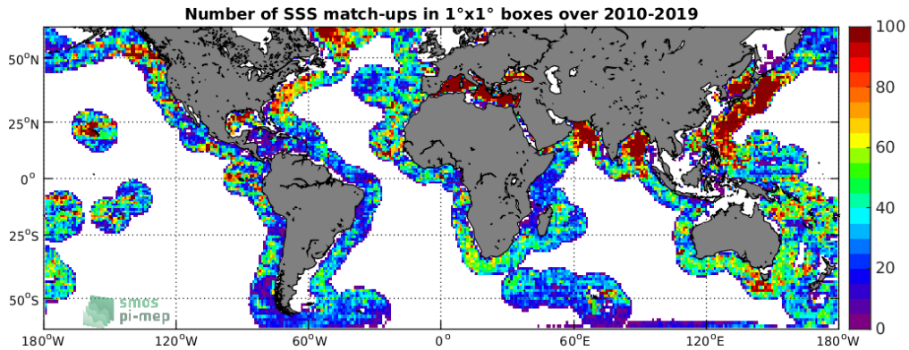
Figure 4: Number of SSS match-ups between Argo SSS and the SMOS-L3-CATDS-CECOS-LOCEAN-V4-9DAYS-25KM SSS product for the SMOS coastal zone ( \approx 800\text{km} ) 60N-60S Pi-MEP region over 1^\circ \times 1^\circ boxes and for the full satellite product period.
