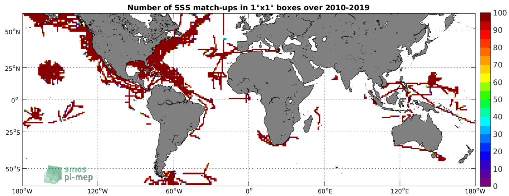
Figure 4: Number of SSS match-ups between TSG-SAMOS SSS and the SMOS-L3-CATDS-CECOS-LOCEAN-V4-18DAYS-25KM SSS product for the SMOS coastal zone (<800km) 60N-60S Pi-MEP region over 1°x1° boxes and for the full satellite product period.
