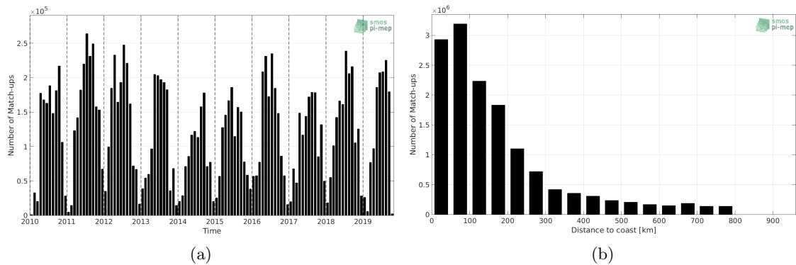
Figure 1: Number of match-ups between TSG-SAMOS and SMOS-L3-CATDS-CECOS-LOCEAN-V4-18DAYS-25KM SSS as a function of time (a) and as function of the distance to coast (b) over the SMOS coastal zone (<800km) 60N-60S Pi-MEP region and for the full satellite product period.
