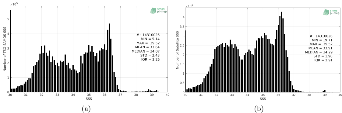
Figure 2: Histograms of SSS from TSG-SAMOS (a) and SMOS-L3-CATDS-CECOS-LOCEAN-V4-18DAYS-25KM (b) considering all match-up pairs per bins of 0.1 over the SMOS coastal zone (<800km) 60N-60S Pi-MEP region and for the full satellite product period.
