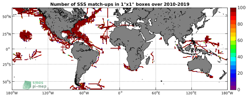
Figure 4: Number of SSS match-ups between TSG-SAMOS SSS and the SMOS-L3-CATDS-CECOS-LOCEAN-V4-18DAYS-25KM SSS product for the SMOS coastal zone ( \approx 800\text{km} ) 60N-60S Pi-MEP region over 1^\circ \times 1^\circ boxes and for the full satellite product period.
