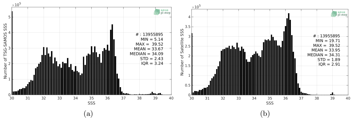
Figure 2: Histograms of SSS from TSG-SAMOS (a) and SMOS-L3-CATDS-CECOS-LOCEAN-V4-18DAYS-25KM (b) considering all match-up pairs per bins of 0.1 over the SMOS coastal zone ( \leq 800 km) 60N-60S Pi-MEP region and for the full satellite product period.
