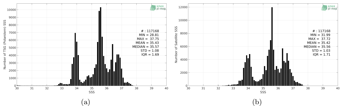
Figure 2: Histograms of SSS from TSG (Polarstern) (a) and SMOS SSS L3 v4 - 18 Days (CATDS-CECOS-LOCEAN) (b) considering all match-up pairs per bins of 0.1 over the SMOS coastal zone (<800km) 60N-60S Pi-MEP region and for the full satellite product period.
