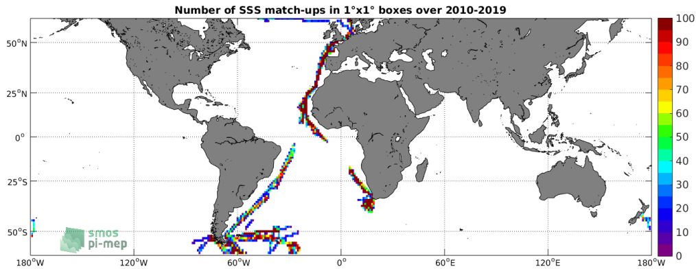
Figure 4: Number of SSS match-ups between TSG (Polarstern) SSS and the SMOS SSS L3 v4 - 18 Days (CATDS-CECOS-LOCEAN) SSS product for the SMOS coastal zone (<800km) 60N-60S Pi-MEP region over 1°x1° boxes and for the full satellite product period.
