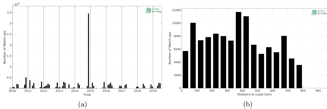
Figure 1: Number of match-ups between TSG (Polarstern) and SMOS SSS L3 v4 - 18 Days (CATDS-CECOS-LOCEAN) SSS as a function of time (a) and as function of the distance to coast (b) over the SMOS coastal zone (<800km) 60N-60S Pi-MEP region and for the full satellite product period.
