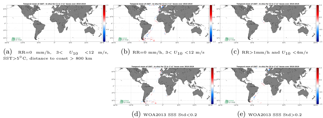
Figure 12: Temporal mean gridded over spatial boxes of size 1^\circ \times 1^\circ of \Delta SSS (SMOS SSS L3 v4 - 18 Days (CATDS-CECOS-LOCEAN) - TSG (Polarstern)) for 5 different subdatasets corresponding to:RR=0 mm/h, 3 < U_{10} < 12 m/s, SST >5^\circ C, distance to coast > 800 km (a), RR=0 mm/h, 3 < U_{10} < 12 m/s (b), RR >1 mm/h and U_{10} < 4 m/s (c), WOA2013 SSS Std <0.2 (d), WOA2013 SSS Std >0.2 (e).
