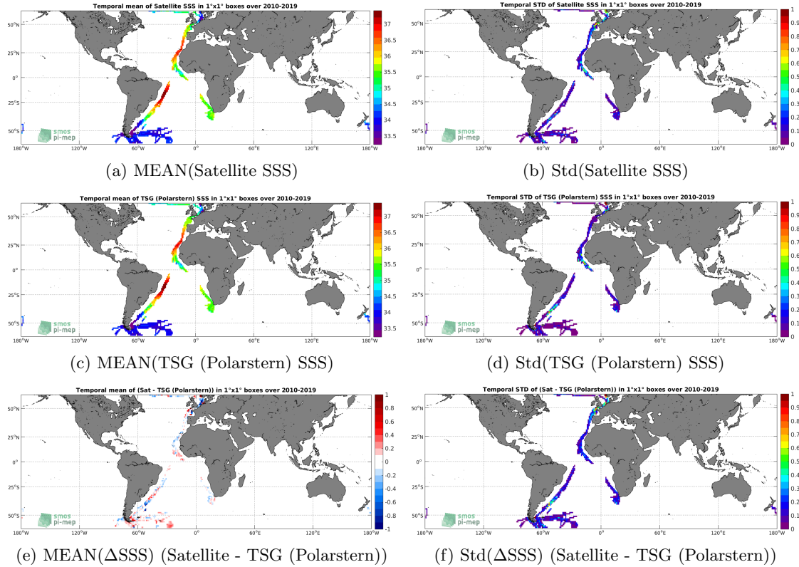
Figure 6: Temporal mean (left) and Std (right) of SSS from SMOS SSS L3 v4 - 18 Days (CATDS-CECOS-LOCEAN) (top), TSG (Polarstern) (middle), and of \Delta SSS (Satellite - TSG (Polarstern)). Only match-up pairs are used to generate these maps.
