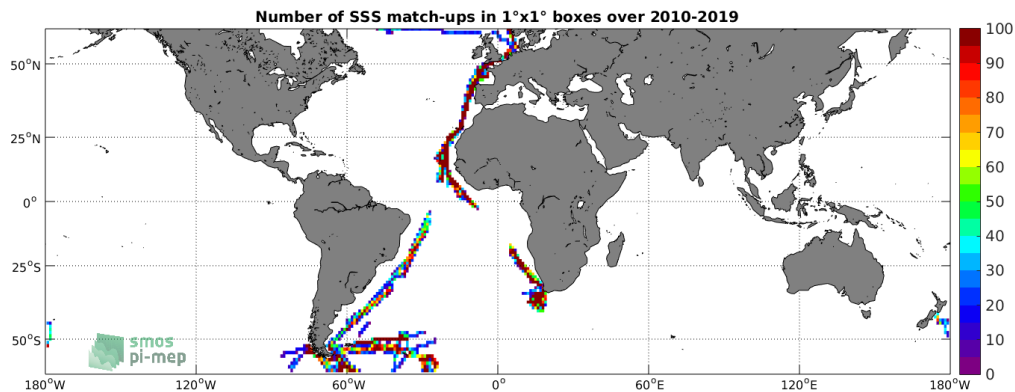
Figure 4: Number of SSS match-ups between TSG-POLARSTERN SSS and the SMOS-L3-CATDS-CECOS-LOCEAN-V4-18DAYS-25KM SSS product for the SMOS coastal zone (<800km) 60N-60S Pi-MEP region over 1^\circ \times 1^\circ boxes and for the full satellite product period.
