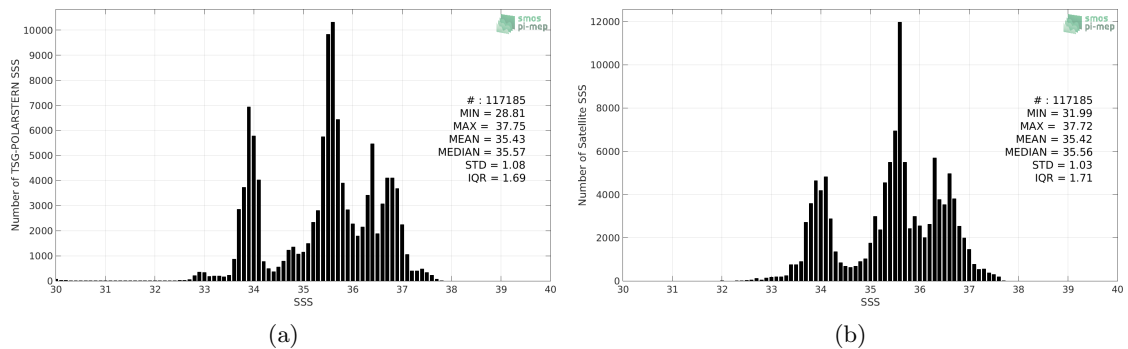
Figure 2: Histograms of SSS from TSG-POLARSTERN (a) and SMOS-L3-CATDS-CECOS-LOCEAN-V4-18DAYS-25KM (b) considering all match-up pairs per bins of 0.1 over the SMOS coastal zone (<800km) 60N-60S Pi-MEP region and for the full satellite product period.
