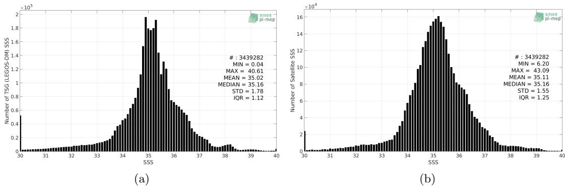
Figure 2: Histograms of SSS from TSG (LEGOS-DM) (a) and SMOS SSS L3 v4 - 18 Days (CATDS-CECOS-LOCEAN) (b) considering all match-up pairs per bins of 0.1 over the SMOS coastal zone (<800km) 60N-60S Pi-MEP region and for the full satellite product period.
