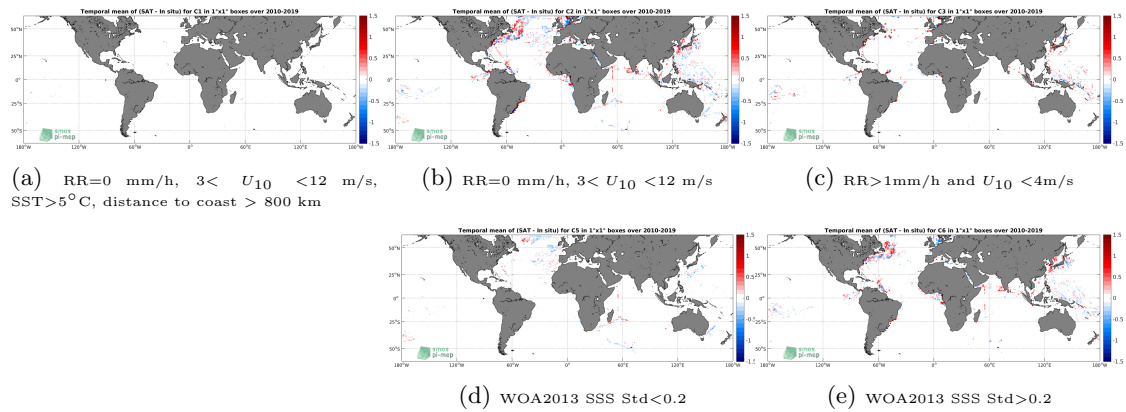
Figure 12: Temporal mean gridded over spatial boxes of size 1^\circ \times 1^\circ of \Delta SSS (SMOS SSS L3 v4 - 18 Days (CATDS-CECOS-LOCEAN) - TSG (LEGOS-DM)) for 5 different subdatasets corresponding to: RR=0 mm/h, 3 < U_{10} < 12 m/s, SST > 5°C, distance to coast > 800 km (a), RR=0 mm/h, 3 < U_{10} < 12 m/s (b), RR > 1mm/h and U_{10} < 4 m/s (c), WOA2013 SSS Std < 0.2 (d), WOA2013 SSS Std > 0.2 (e).
