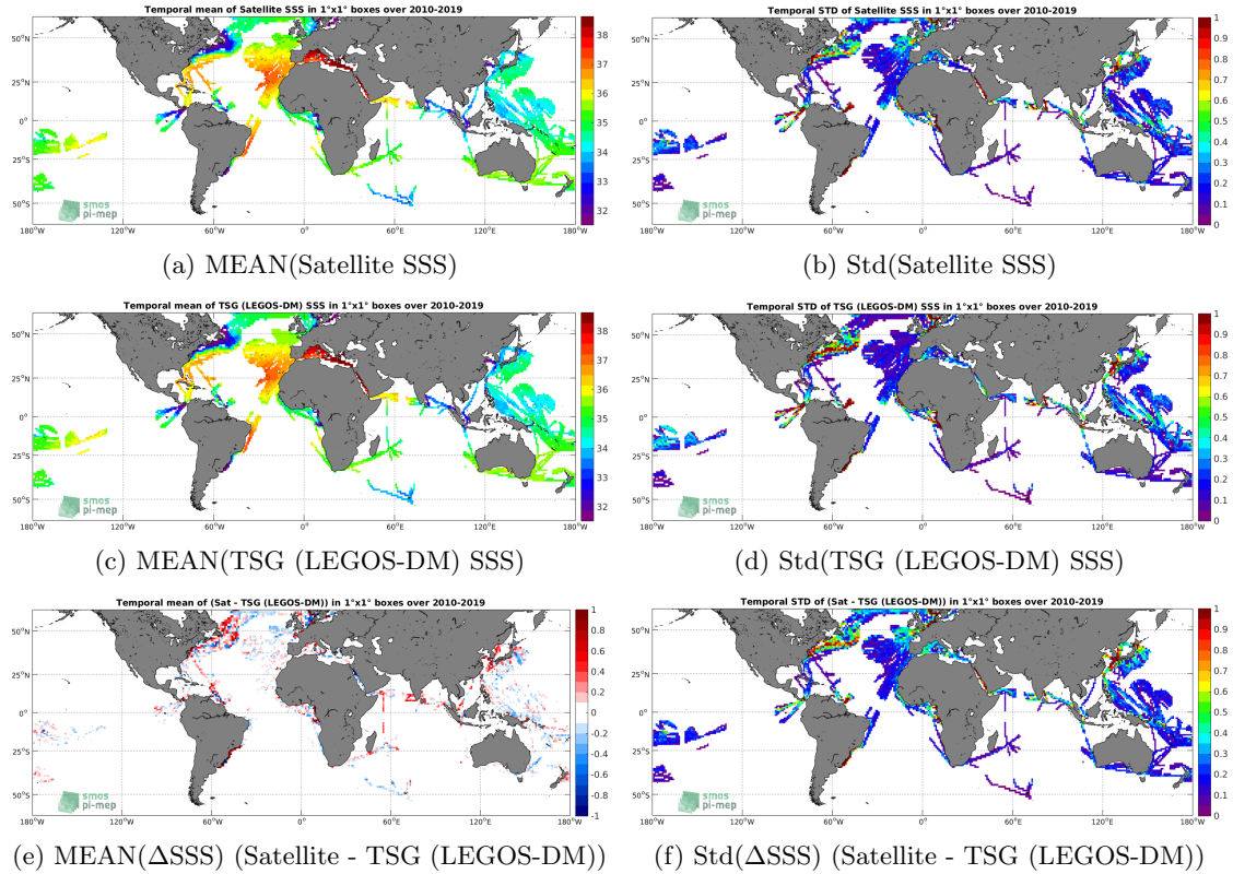
Figure 6: Temporal mean (left) and Std (right) of SSS from SMOS SSS L3 v4 - 18 Days (CATDS-CECOS-LOCEAN) (top), TSG (LEGOS-DM) (middle), and of \Delta SSS (Satellite - TSG (LEGOS-DM)). Only match-up pairs are used to generate these maps.
