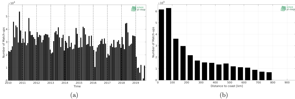
Figure 1: Number of match-ups between TSG (LEGOS-DM) and SMOS SSS L3 v4 - 18 Days (CATDS-CECOS-LOCEAN) SSS as a function of time (a) and as function of the distance to coast (b) over the SMOS coastal zone (<800km) 60N-60S Pi-MEP region and for the full satellite product period.
