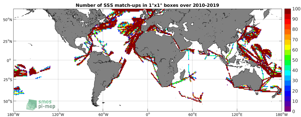
Figure 4: Number of SSS match-ups between TSG-LEGOS-DM SSS and the SMOS-L3-CATDS-CECOS-LOCEAN-V4-18DAYS-25KM SSS product for the SMOS coastal zone (<800km) 60N-60S Pi-MEP region over 1^\circ \times 1^\circ boxes and for the full satellite product period.
