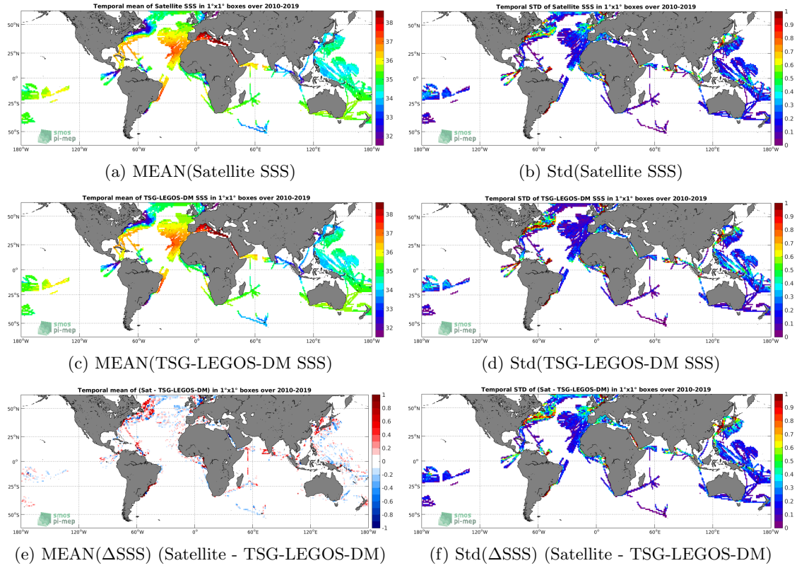
Figure 6: Temporal mean (left) and Std (right) of SSS from SMOS-L3-CATDS-CECOS-LOCEAN-V4-18DAYS-25KM (top), TSG-LEGOS-DM (middle), and of \Delta SSS (Satellite - TSG-LEGOS-DM). Only match-up pairs are used to generate these maps.
