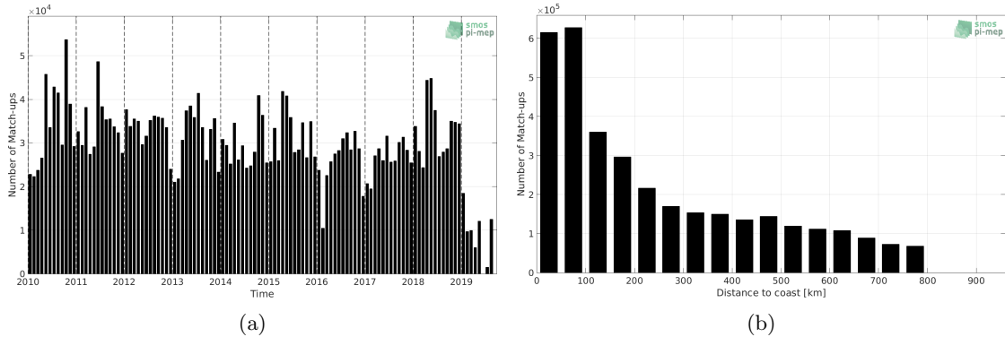
Figure 1: Number of match-ups between TSG-LEGOS-DM and SMOS-L3-CATDS-CECOS-LOCEAN-V4-18DAYS-25KM SSS as a function of time (a) and as function of the distance to coast (b) over the SMOS coastal zone (<800km) 60N-60S Pi-MEP region and for the full satellite product period.
