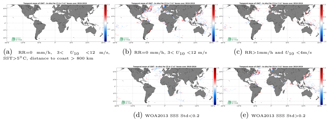
Figure 12: Temporal mean gridded over spatial boxes of size 1^\circ \times 1^\circ of \Delta SSS (SMOS-L3-CATDS-CECOS-LOCEAN-V4-18DAYS-25KM - TSG-LEGOS-DM) for 5 different subdatasets corresponding to:RR=0 mm/h, 3 < U_{10} < 12 m/s, SST >5^\circ C, distance to coast > 800 km (a), RR=0 mm/h, 3 < U_{10} < 12 m/s (b), RR >1 mm/h and U_{10} < 4 m/s (c), WOA2013 SSS Std <0.2 (d), WOA2013 SSS Std >0.2 (e).
