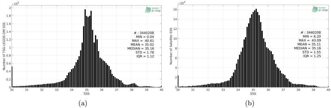
Figure 2: Histograms of SSS from TSG-LEGOS-DM (a) and SMOS-L3-CATDS-CECOS-LOCEAN-V4-18DAYS-25KM (b) considering all match-up pairs per bins of 0.1 over the SMOS coastal zone (<800km) 60N-60S Pi-MEP region and for the full satellite product period.
