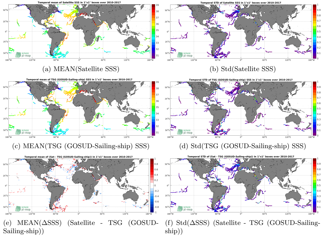
Figure 6: Temporal mean (left) and Std (right) of SSS from SMOS SSS L3 v4 - 18 Days (CATDS-CECOS-LOCEAN) (top), TSG (GOSUD-Sailing-ship) (middle), and of \Delta SSS (Satellite - TSG (GOSUD-Sailing-ship)). Only match-up pairs are used to generate these maps.
