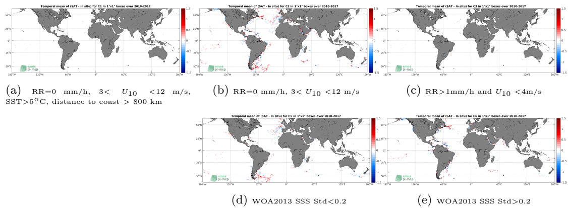
Figure 12: Temporal mean gridded over spatial boxes of size 1^\circ \times 1^\circ of \Delta\text{SSS} (SMOS SSS L3 v4 - 18 Days (CATDS-CECOS-LOCEAN) - TSG (GOSUD-Sailing-ship)) for 5 different subdatasets corresponding to: RR=0 mm/h, 3 < U_{10} < 12 m/s, SST > 5°C, distance to coast > 800 km (a), RR=0 mm/h, 3 < U_{10} < 12 m/s (b), RR > 1mm/h and U_{10} < 4 m/s (c), WOA2013 SSS Std < 0.2 (d), WOA2013 SSS Std > 0.2 (e).
