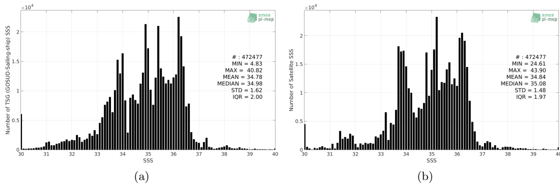
Figure 2: Histograms of SSS from TSG (GOSUD-Sailing-ship) (a) and SMOS SSS L3 v4 - 18 Days (CATDS-CECOS-LOCEAN) (b) considering all match-up pairs per bins of 0.1 over the SMOS coastal zone (<800km) 60N-60S Pi-MEP region and for the full satellite product period.
