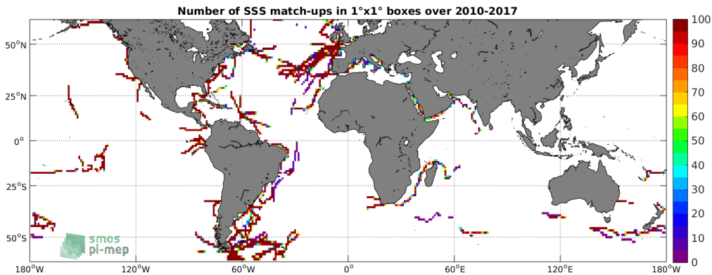
Figure 4: Number of SSS match-ups between TSG (GOSUD-Sailing-ship) SSS and the SMOS SSS L3 v4 - 18 Days (CATDS-CECOS-LOCEAN) SSS product for the SMOS coastal zone (<800km) 60N-60S Pi-MEP region over 1^\circ \times 1^\circ boxes and for the full satellite product period.
