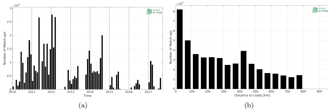
Figure 1: Number of match-ups between TSG (GOSUD-Sailing-ship) and SMOS SSS L3 v4 - 18 Days (CATDS-CECOS-LOCEAN) SSS as a function of time (a) and as function of the distance to coast (b) over the SMOS coastal zone (<800km) 60N-60S Pi-MEP region and for the full satellite product period.
