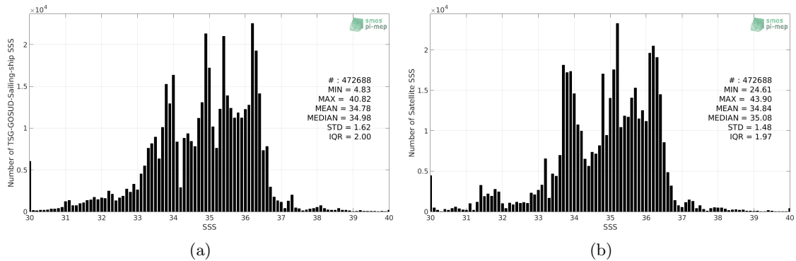
Figure 2: Histograms of SSS from TSG-GOSUD-Sailing-ship (a) and SMOS-L3-CATDS-CECOS-LOCEAN-V4-18DAYS-25KM (b) considering all match-up pairs per bins of 0.1 over the SMOS coastal zone (<800km) 60N-60S Pi-MEP region and for the full satellite product period.
