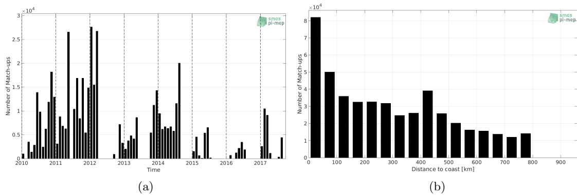
Figure 1: Number of match-ups between TSG-GOSUD-Sailing-ship and SMOS-L3-CATDS-CECOS-LOCEAN-V4-18DAYS-25KM SSS as a function of time (a) and as function of the distance to coast (b) over the SMOS coastal zone (<800km) 60N-60S Pi-MEP region and for the full satellite product period.
