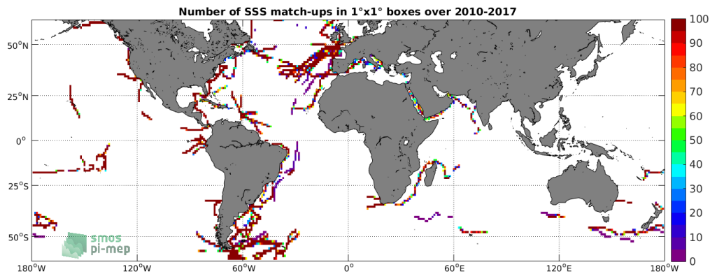
Figure 4: Number of SSS match-ups between TSG-GOSUD-Sailing-ship SSS and the SMOS-L3-CATDS-CECOS-LOCEAN-V4-18DAYS-25KM SSS product for the SMOS coastal zone (<800km) 60N-60S Pi-MEP region over 1°x1° boxes and for the full satellite product period.
