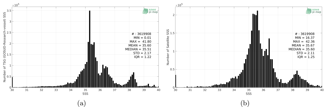
Figure 2: Histograms of SSS from TSG (GOSUD-Research-vessel) (a) and SMOS SSS L3 v4 - 18 Days (CATDS-CECOS-LOCEAN) (b) considering all match-up pairs per bins of 0.1 over the SMOS coastal zone (<800km) 60N-60S Pi-MEP region and for the full satellite product period.
