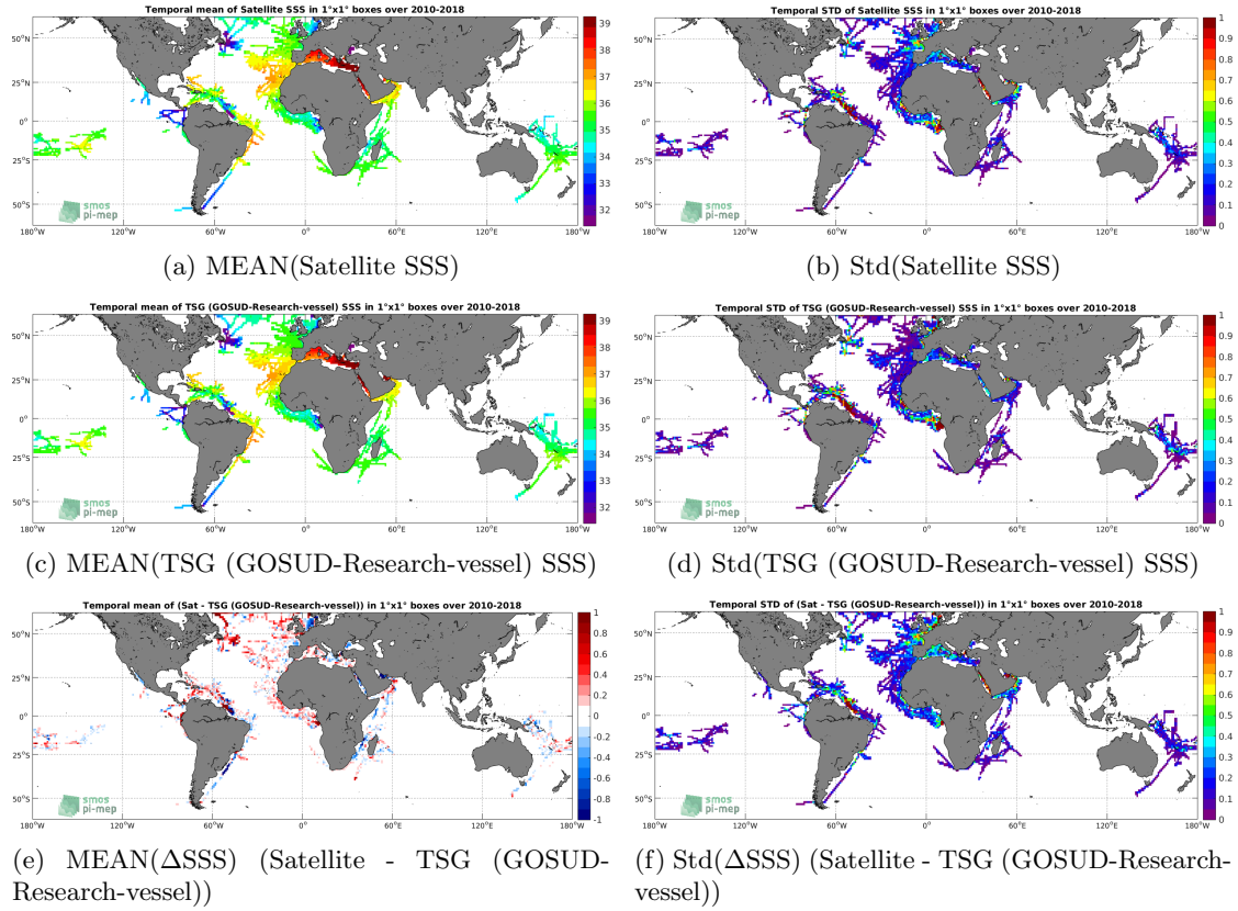
Figure 6: Temporal mean (left) and Std (right) of SSS from SMOS SSS L3 v4 - 18 Days (CATDS-CECOS-LOCEAN) (top), TSG (GOSUD-Research-vessel) (middle), and of \Delta SSS (Satellite - TSG (GOSUD-Research-vessel)). Only match-up pairs are used to generate these maps.
