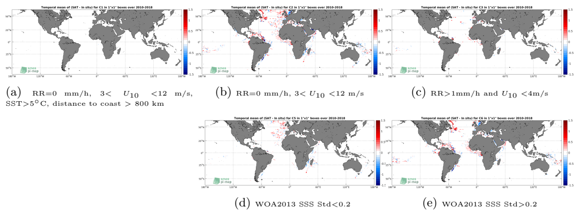
Figure 12: Temporal mean gridded over spatial boxes of size 1^\circ \times 1^\circ of \Delta SSS (SMOS SSS L3 v4 - 18 Days (CATDS-CECOS-LOCEAN) - TSG (GOSUD-Research-vessel)) for 5 different subdatasets corresponding to:RR=0 mm/h, 3 < U_{10} < 12 m/s, SST>5°C, distance to coast > 800 km (a), RR=0 mm/h, 3 < U_{10} < 12 m/s (b), RR>1mm/h and U_{10} < 4 m/s (c), WOA2013 SSS Std<0.2 (d), WOA2013 SSS Std>0.2 (e).
