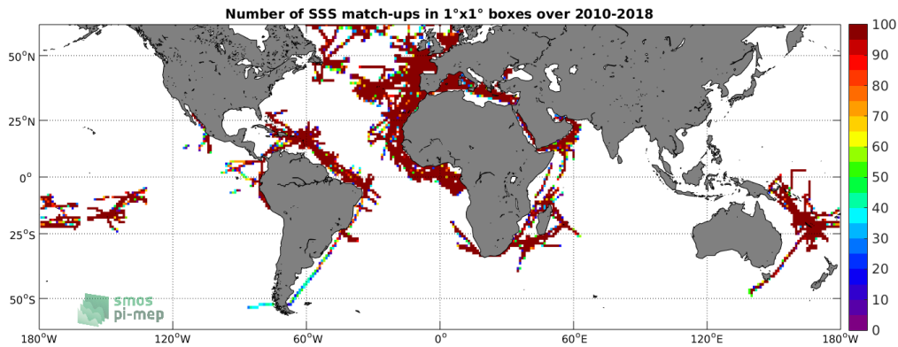
Figure 4: Number of SSS match-ups between TSG (GOSUD-Research-vessel) SSS and the SMOS SSS L3 v4 - 18 Days (CATDS-CECOS-LOCEAN) SSS product for the SMOS coastal zone (<800km) 60N-60S Pi-MEP region over 1^\circ \times 1^\circ boxes and for the full satellite product period.
