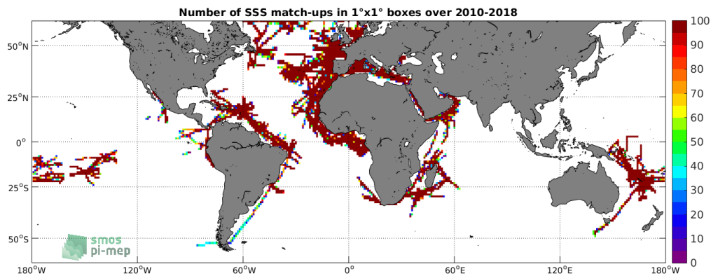
Figure 4: Number of SSS match-ups between TSG-GOSUD-Research-vessel SSS and the SMOS-L3-CATDS-CECOS-LOCEAN-V4-18DAYS-25KM SSS product for the SMOS coastal zone (<800km) 60N-60S Pi-MEP region over 1^\circ \times 1^\circ boxes and for the full satellite product period.
