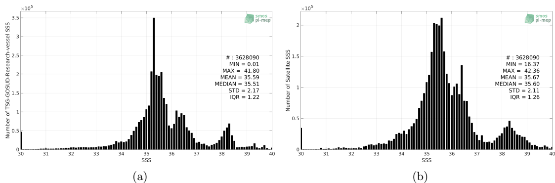
Figure 2: Histograms of SSS from TSG-GOSUD-Research-vessel (a) and SMOS-L3-CATDS-CECOS-LOCEAN-V4-18DAYS-25KM (b) considering all match-up pairs per bins of 0.1 over the SMOS coastal zone (<800km) 60N-60S Pi-MEP region and for the full satellite product period.
