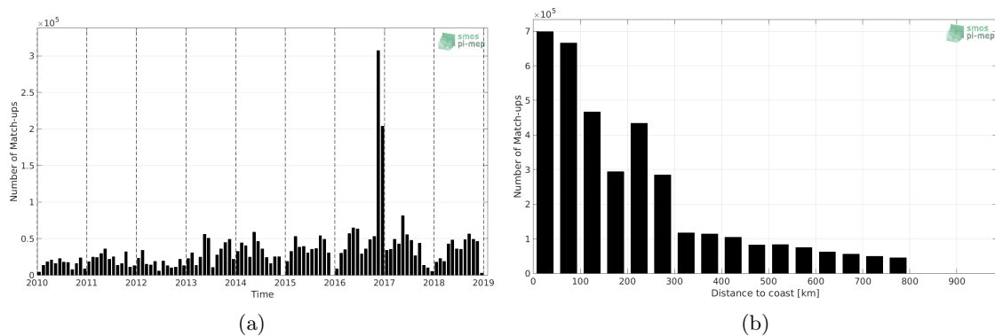
Figure 1: Number of match-ups between TSG-GOSUD-Research-vessel and SMOS-L3-CATDS-CECOS-LOCEAN-V4-18DAYS-25KM SSS as a function of time (a) and as function of the distance to coast (b) over the SMOS coastal zone (<800km) 60N-60S Pi-MEP region and for the full satellite product period.
