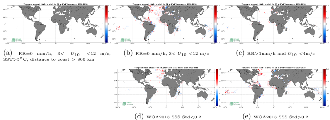
Figure 12: Temporal mean gridded over spatial boxes of size 1^\circ \times 1^\circ of \Delta SSS (SMOS-L3-CATDS-CECOS-LOCEAN-V4-18DAYS-25KM - TSG-GOSUD-Research-vessel) for 5 different subdatasets corresponding to:RR=0 mm/h, 3 < U_{10} < 12 m/s, SST >5^\circ C, distance to coast > 800 km (a), RR=0 mm/h, 3 < U_{10} < 12 m/s (b), RR >1 mm/h and U_{10} < 4 m/s (c), WOA2013 SSS Std <0.2 (d), WOA2013 SSS Std >0.2 (e).
