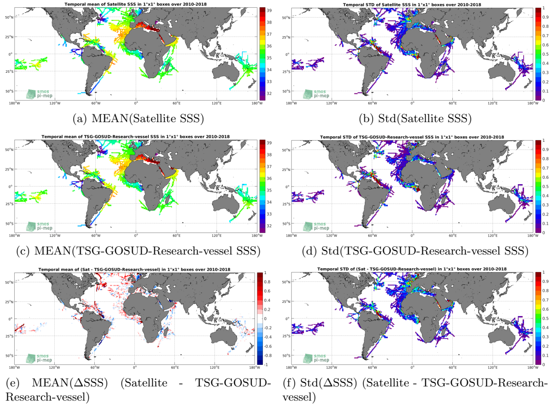
Figure 6: Temporal mean (left) and Std (right) of SSS from SMOS-L3-CATDS-CECOS-LOCEAN-V4-18DAYS-25KM (top), TSG-GOSUD-Research-vessel (middle), and of \Delta SSS (Satellite - TSG-GOSUD-Research-vessel). Only match-up pairs are used to generate these maps.
