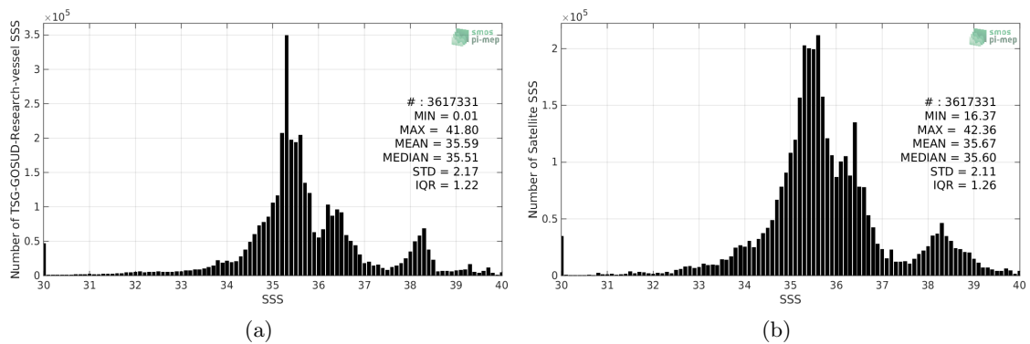
Figure 2: Histograms of SSS from TSG-GOSUD-Research-vessel (a) and SMOS-L3-CATDS-CECOS-LOCEAN-V4-18DAYS-25KM (b) considering all match-up pairs per bins of 0.1 over the SMOS coastal zone ( \geq 800 km) 60N-60S Pi-MEP region and for the full satellite product period.
