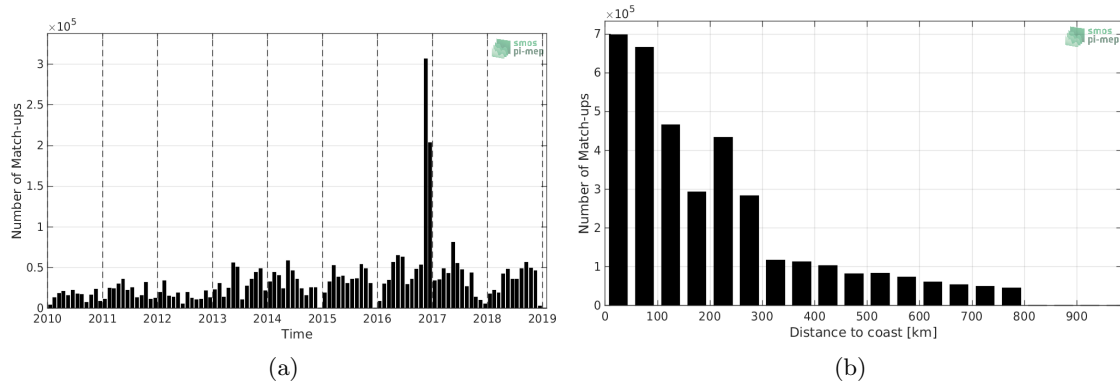
Figure 1: Number of match-ups between TSG-GOSUD-Research-vessel and SMOS-L3-CATDS-CECOS-LOCEAN-V4-18DAYS-25KM SSS as a function of time (a) and as function of the distance to coast (b) over the SMOS coastal zone ( \geq 800 km) 60N-60S Pi-MEP region and for the full satellite product period.
