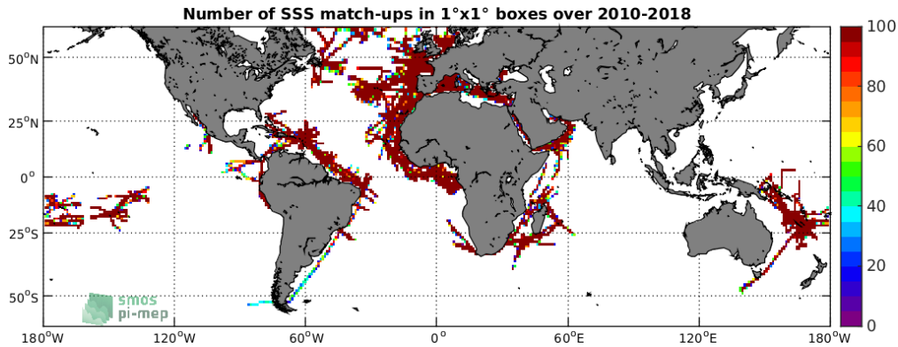
Figure 4: Number of SSS match-ups between TSG-GOSUD-Research-vessel SSS and the SMOS-L3-CATDS-CECOS-LOCEAN-V4-18DAYS-25KM SSS product for the SMOS coastal zone ( \approx 800\text{km} ) 60N-60S Pi-MEP region over 1^\circ \times 1^\circ boxes and for the full satellite product period.
