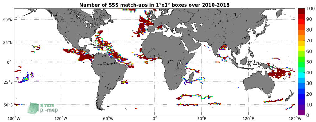
Figure 3: Number of SSS match-ups between Surface drifters SSS and the SMOS-L3-CATDS-CECOS-LOCEAN-V4-18DAYS-25KM SSS product for the SMOS coastal zone (<800km) 60N-60S Pi-MEP region over 1°x1° boxes and for the full satellite product period.
