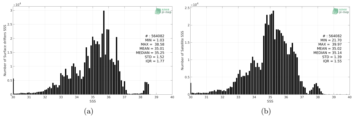
Figure 2: Histograms of SSS from Surface drifters (a) and SMOS-L3-CATDS-CECOS-LOCEAN-V4-18DAYS-25KM (b) considering all match-up pairs per bins of 0.1 over the SMOS coastal zone (<800km) 60N-60S Pi-MEP region and for the full satellite product period.
