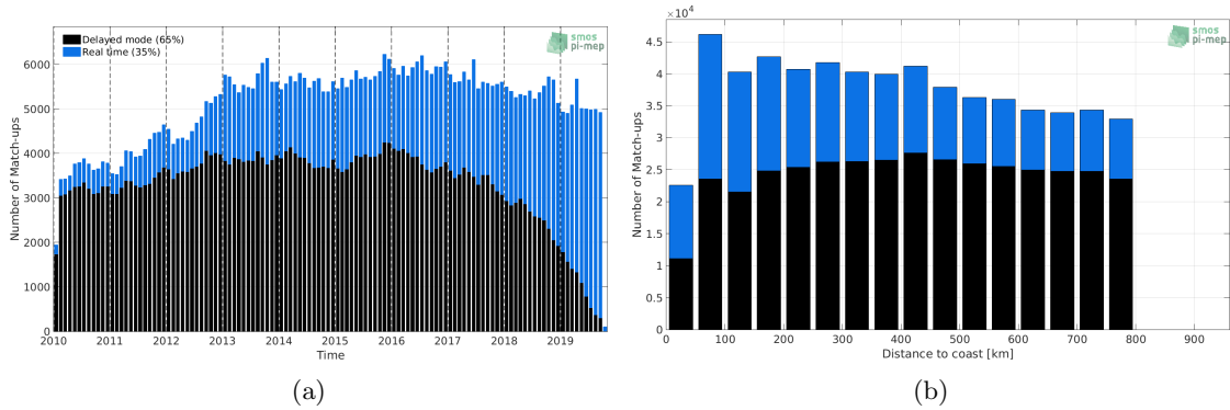
Figure 1: Number of match-ups between Argo and SMOS-L3-CATDS-CECOS-LOCEAN-V4-18DAYS-25KM SSS as a function of time (a) and as function of the distance to coast (b) over the SMOS coastal zone (<800km) 60N-60S Pi-MEP region and for the full satellite product period.
