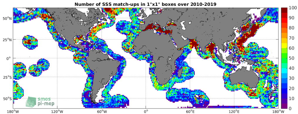
Figure 4: Number of SSS match-ups between Argo SSS and the SMOS-L3-CATDS-CECOS-LOCEAN-V4-18DAYS-25KM SSS product for the SMOS coastal zone (<800km) 60N-60S Pi-MEP region over 1°x1° boxes and for the full satellite product period.
