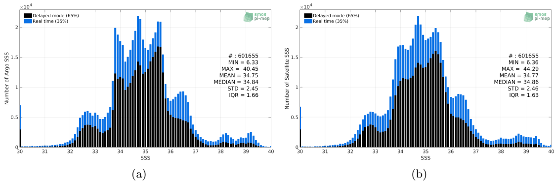
Figure 2: Histograms of SSS from Argo (a) and SMOS-L3-CATDS-CECOS-LOCEAN-V4-18DAYS-25KM (b) considering all match-up pairs per bins of 0.1 over the SMOS coastal zone (<800km) 60N-60S Pi-MEP region and for the full satellite product period.
