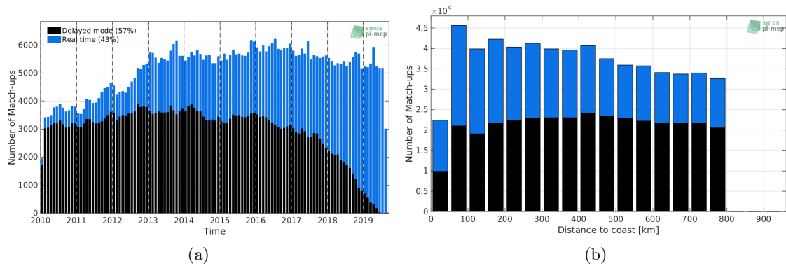
Figure 1: Number of match-ups between Argo and SMOS-L3-CATDS-CECOS-LOCEAN-V4-18DAYS-25KM SSS as a function of time (a) and as function of the distance to coast (b) over the SMOS coastal zone (j800km) 60N-60S Pi-MEP region and for the full satellite product period.
