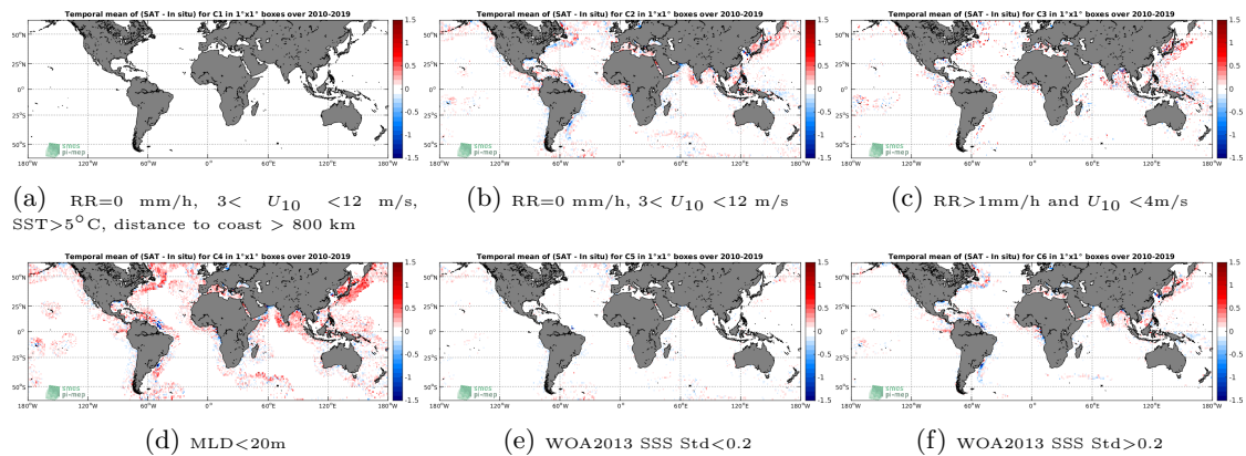
Figure 12: Temporal mean gridded over spatial boxes of size 1^\circ \times 1^\circ of \Delta SSS (SMOS-L3-CATDS-CECOS-LOCEAN-V4-18DAYS-25KM - Argo) for 6 different subdatasets corresponding to:RR=0 mm/h, 3 < U_{10} < 12 m/s, SST >5^\circ C, distance to coast > 800 km (a), RR=0 mm/h, 3 < U_{10} < 12 m/s (b), RR >1 mm/h and U_{10} < 4 m/s (c),MLD <20 m (d),WOA2013 SSS Std <0.2 (e),WOA2013 SSS Std >0.2 (f).
