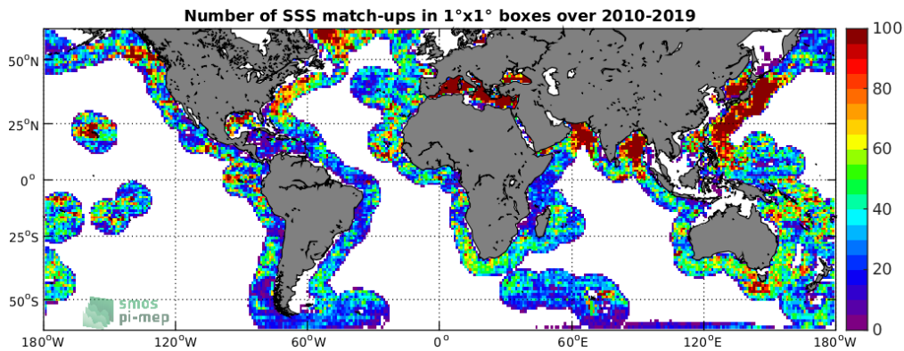
Figure 4: Number of SSS match-ups between Argo SSS and the SMOS-L3-CATDS-CECOS-LOCEAN-V4-18DAYS-25KM SSS product for the SMOS coastal zone ( \geq 800\text{km} ) 60N-60S Pi-MEP region over 1^\circ \times 1^\circ boxes and for the full satellite product period.
