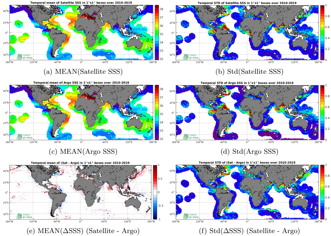
Figure 6: Temporal mean (left) and Std (right) of SSS from SMOS-L3-CATDS-CECOS-LOCEAN-V4-18DAYS-25KM (top), Argo (middle), and of \Delta SSS (Satellite - Argo). Only match-up pairs are used to generate these maps.
