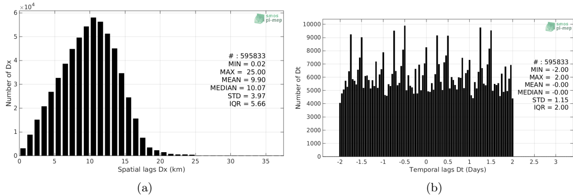
Figure 5: Histograms of the spatial (a) and temporal (b) lags between the time of the Argo measurements and the date of the corresponding SMOS-L3-CATDS-CECOS-LOCEAN-V4-18DAYS-25KM SSS product.
