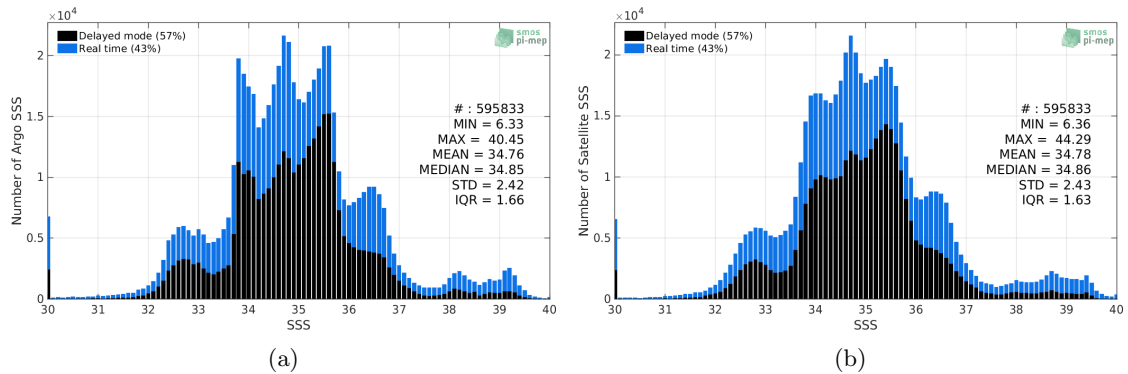
Figure 2: Histograms of SSS from Argo (a) and SMOS-L3-CATDS-CECOS-LOCEAN-V4-18DAYS-25KM (b) considering all match-up pairs per bins of 0.1 over the SMOS coastal zone (j800km) 60N-60S Pi-MEP region and for the full satellite product period.
