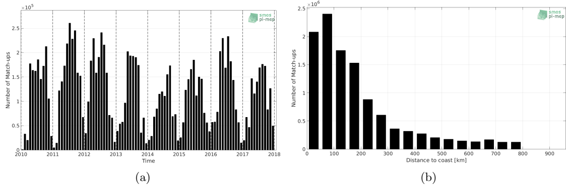
Figure 1: Number of match-ups between TSG-SAMOS and SMOS-L3-CATDS-CECOS-LOCEAN-V3-9DAYS-25KM SSS as a function of time (a) and as function of the distance to coast (b) over the SMOS coastal zone ( \pm 800 km) 60N-60S Pi-MEP region and for the full satellite product period.
