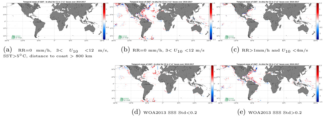
Figure 12: Temporal mean gridded over spatial boxes of size 1^\circ \times 1^\circ of \Delta SSS (SMOS-L3-CATDS-CECOS-LOCEAN-V3-9DAYS-25KM - TSG-SAMOS) for 5 different subdatasets corresponding to: RR=0 mm/h, 3 < U_{10} < 12 m/s, SST > 5^\circ C , distance to coast > 800 km (a), RR=0 mm/h, 3 < U_{10} < 12 m/s (b), RR > 1 mm/h and U_{10} < 4 m/s (c), WOA2013 SSS Std < 0.2 (d), WOA2013 SSS Std > 0.2 (e).
