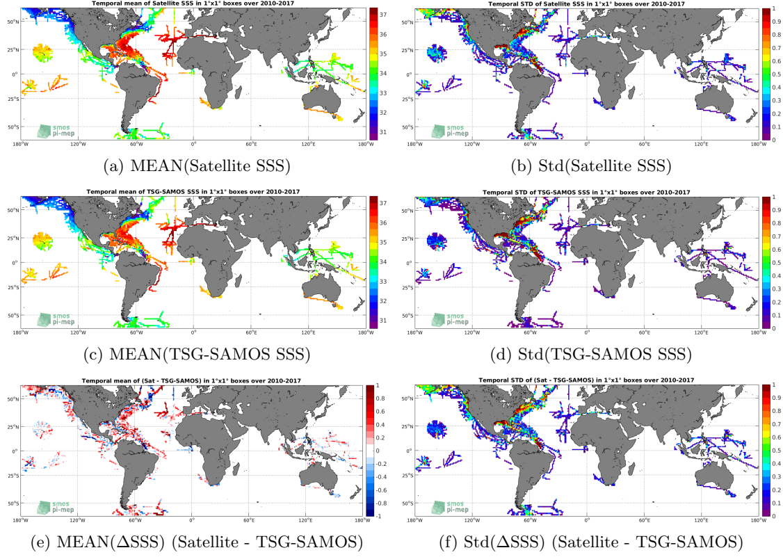
Figure 6: Temporal mean (left) and Std (right) of SSS from SMOS-L3-CATDS-CECOS-LOCEAN-V3-9DAYS-25KM (top), TSG-SAMOS (middle), and of \Delta SSS (Satellite - TSG-SAMOS). Only match-up pairs are used to generate these maps.
