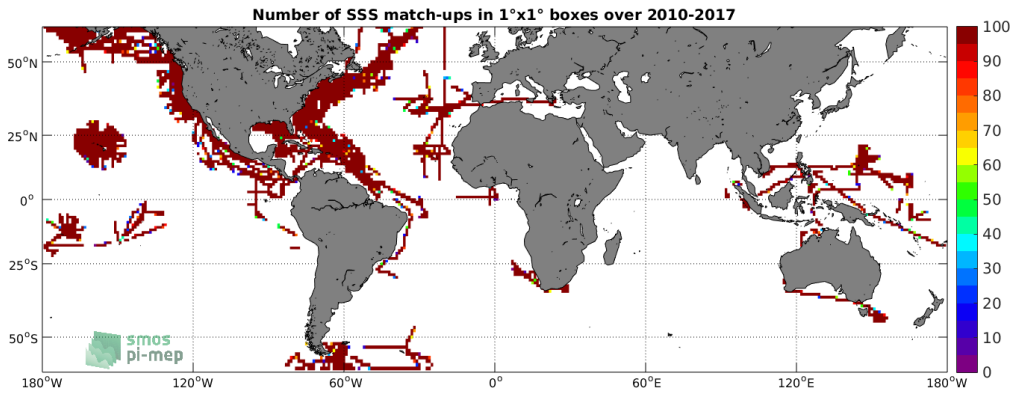
Figure 4: Number of SSS match-ups between TSG-SAMOS SSS and the SMOS-L3-CATDS-CECOS-LOCEAN-V3-9DAYS-25KM SSS product for the SMOS coastal zone ( \geq 800\text{km} ) 60^\circ\text{N} - 60^\circ\text{S} Pi-MEP region over 1^\circ \times 1^\circ boxes and for the full satellite product period.
