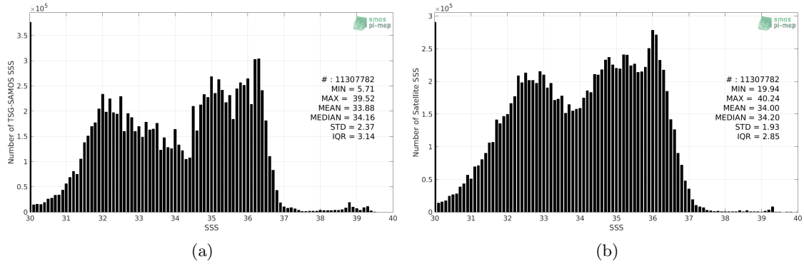
Figure 2: Histograms of SSS from TSG-SAMOS (a) and SMOS-L3-CATDS-CECOS-LOCEAN-V3-9DAYS-25KM (b) considering all match-up pairs per bins of 0.1 over the SMOS coastal zone ( \pm 800 km) 60N-60S Pi-MEP region and for the full satellite product period.
