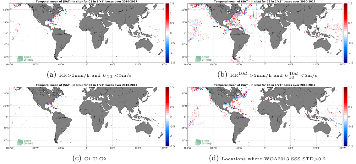
Figure 12: Temporal mean gridded over spatial boxes of size 1^\circ \times 1^\circ of \Delta SSS (SMOS-L3-CATDS-CECOS-LOCEAN-V3-9DAYS-25KM - TSG-SAMOS) for 4 different subdatasets corresponding to: RR > 1mm/h and U_{10} < 5\text{m/s} (a), RR^{10d} > 5\text{mm/h} and U_{10}^{10d} < 5\text{m/s} (b), C1 U C2 (c), Locations where WOA2013 SSS STD > 0.2 (d).
