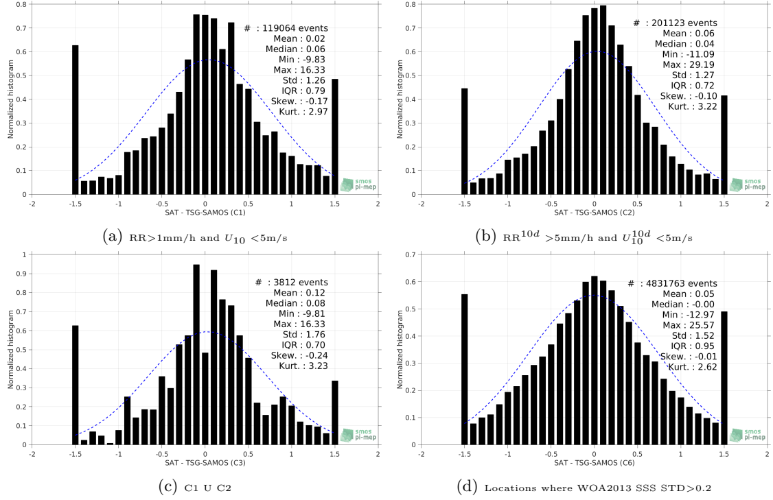
Figure 13: Normalized histogram of \Delta SSS (SMOS-L3-CATDS-CECOS-LOCEAN-V3-9DAYS-25KM - TSG-SAMOS) for 6 different subdatasets corresponding to: RR > 1\text{mm/h} and U_{10} < 5\text{m/s} (a), RR^{10d} > 5\text{mm/h} and U_{10}^{10d} < 5\text{m/s} (b), C1 U C2 (c), Locations where WOA2013 SSS STD > 0.2 (d).
