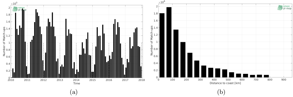
Figure 1: Number of match-ups between TSG-SAMOS and SMOS-L3-CATDS-CECOS-LOCEAN-V3-9DAYS-25KM SSS as a function of time (a) and as function of the distance to coast (b) over the SMOS coastal zone ( \leq 800 km) 60N-60S Pi-MEP region and for the full satellite product period.
