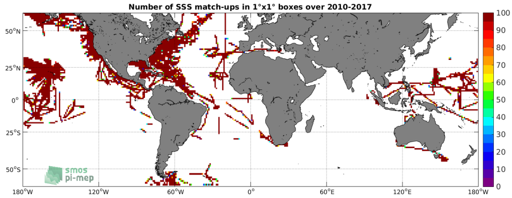
Figure 4: Number of SSS match-ups between TSG-SAMOS SSS and the SMOS-L3-CATDS-CECOS-LOCEAN-V3-9DAYS-25KM SSS product for the SMOS coastal zone ( \delta 800\text{km} ) 60N-60S Pi-MEP region over 1^\circ \times 1^\circ boxes and for the full satellite product period.
