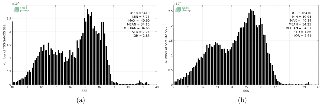
Figure 2: Histograms of SSS from TSG-SAMOS (a) and SMOS-L3-CATDS-CECOS-LOCEAN-V3-9DAYS-25KM (b) considering all match-up pairs per bins of 0.1 over the SMOS coastal zone ( \leq 800 km) 60N-60S Pi-MEP region and for the full satellite product period.
