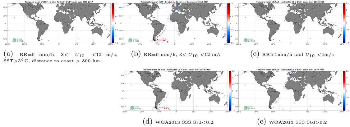
Figure 12: Temporal mean gridded over spatial boxes of size 1^\circ \times 1^\circ of \Delta SSS (SMOS-L3-CATDS-CECOS-LOCEAN-V3-9DAYS-25KM - TSG-POLARSTERN) for 5 different subdatasets corresponding to: RR=0 mm/h, 3 < U_{10} < 12 m/s, SST > 5^\circ C , distance to coast > 800 km (a), RR=0 mm/h, 3 < U_{10} < 12 m/s (b), RR > 1 mm/h and U_{10} < 4 m/s (c), WOA2013 SSS Std < 0.2 (d), WOA2013 SSS Std > 0.2 (e).
