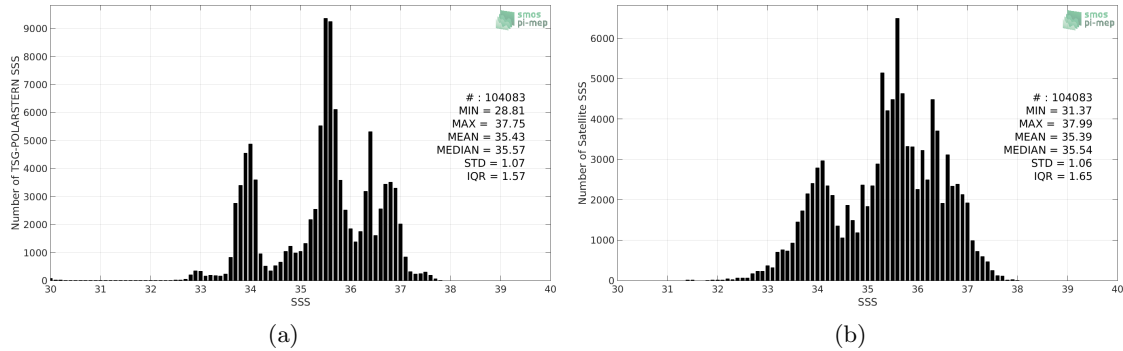
Figure 2: Histograms of SSS from TSG-POLARSTERN (a) and SMOS-L3-CATDS-CECOS-LOCEAN-V3-9DAYS-25KM (b) considering all match-up pairs per bins of 0.1 over the SMOS coastal zone ( \pm 800 km) 60N-60S Pi-MEP region and for the full satellite product period.
