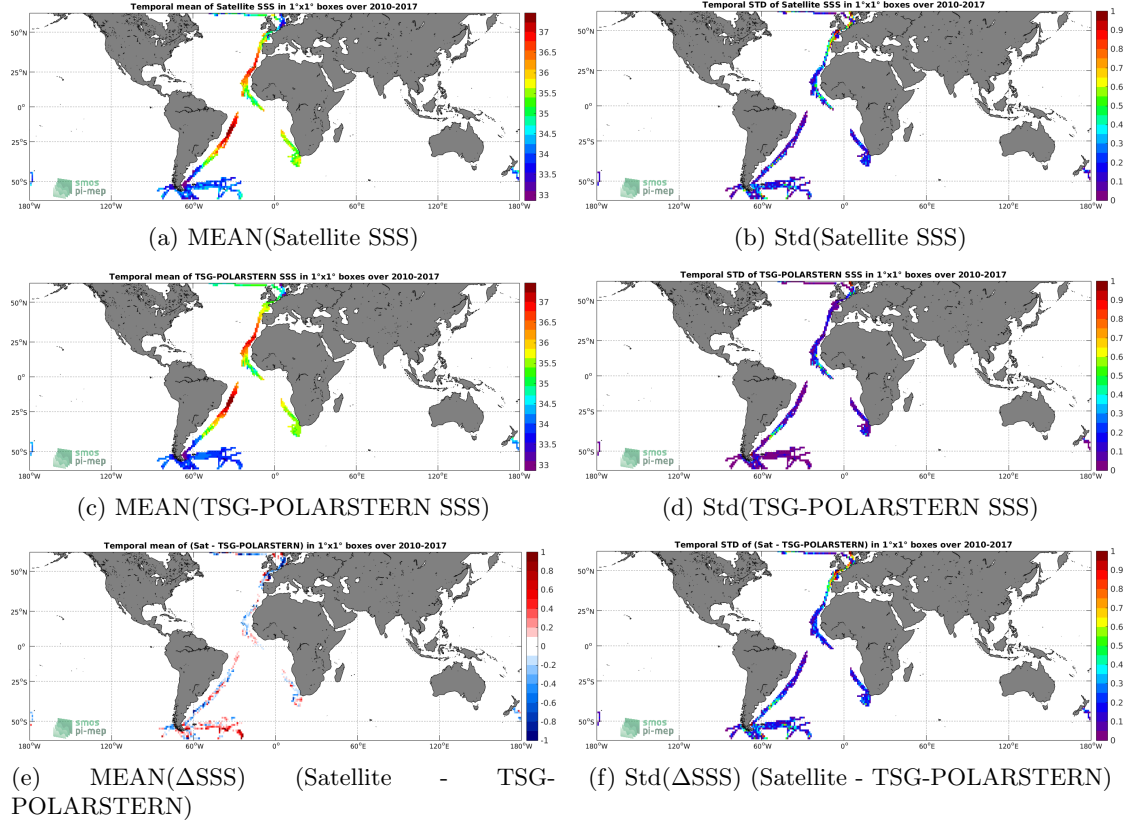
Figure 6: Temporal mean (left) and Std (right) of SSS from SMOS-L3-CATDS-CECOS-LOCEAN-V3-9DAYS-25KM (top), TSG-POLARSTERN (middle), and of \Delta SSS (Satellite - TSG-POLARSTERN). Only match-up pairs are used to generate these maps.
