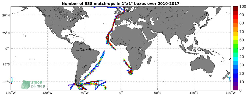
Figure 4: Number of SSS match-ups between TSG-POLARSTERN SSS and the SMOS-L3-CATDS-CECOS-LOCEAN-V3-9DAYS-25KM SSS product for the SMOS coastal zone ( \approx 800 km) 60N-60S Pi-MEP region over 1°x1° boxes and for the full satellite product period.
