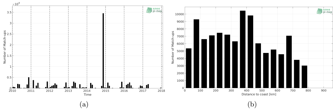
Figure 1: Number of match-ups between TSG-POLARSTERN and SMOS-L3-CATDS-CECOS-LOCEAN-V3-9DAYS-25KM SSS as a function of time (a) and as function of the distance to coast (b) over the SMOS coastal zone ( \pm 800 km) 60N-60S Pi-MEP region and for the full satellite product period.
