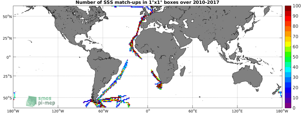
Figure 4: Number of SSS match-ups between TSG-POLARSTERN SSS and the SMOS-L3-CATDS-CECOS-LOCEAN-V3-9DAYS-25KM SSS product for the SMOS coastal zone ( \pm 800\text{km} ) 60N-60S Pi-MEP region over 1^\circ \times 1^\circ boxes and for the full satellite product period.
