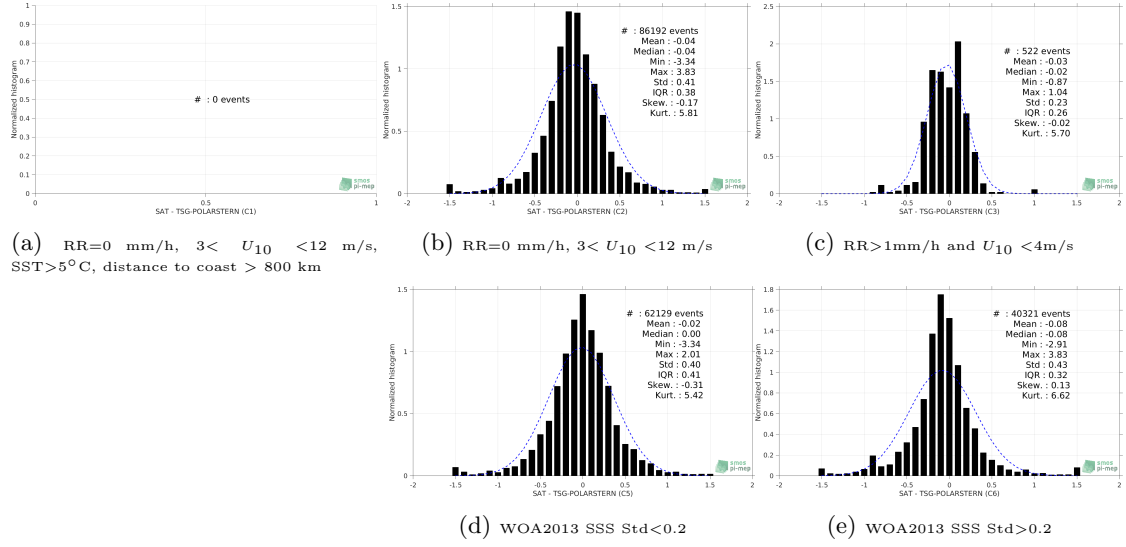
Figure 13: Normalized histogram of \Delta SSS (SMOS-L3-CATDS-CECOS-LOCEAN-V3-9DAYS-25KM - TSG-POLARSTERN) for 5 different subdatasets corresponding to: RR=0 mm/h, 3 < U_{10} < 12 m/s, SST > 5°C, distance to coast > 800 km (a), RR=0 mm/h, 3 < U_{10} < 12 m/s (b), RR > 1mm/h and U_{10} < 4 m/s (c), WOA2013 SSS Std < 0.2 (d), WOA2013 SSS Std > 0.2 (e).
