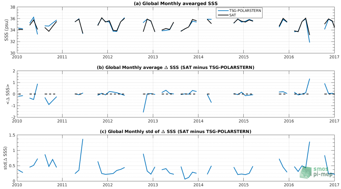
Figure 7: Time series of the monthly averaged mean SSS (top), mean \Delta SSS (Satellite - TSG-POLARSTERN) and Std of \Delta SSS (Satellite - TSG-POLARSTERN) over the SMOS coastal zone ( \pm 800 km) 60N-60S Pi-MEP region considering all match-ups collected by the Pi-MEP platform.
