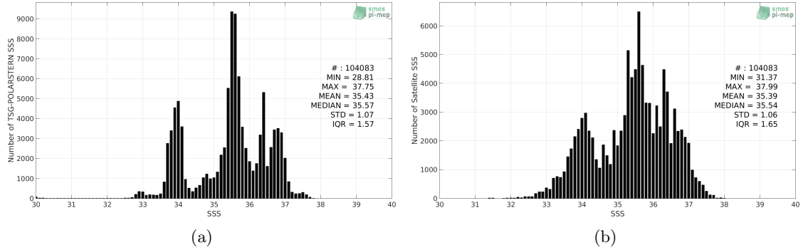
Figure 2: Histograms of SSS from TSG-POLARSTERN (a) and SMOS-L3-CATDS-CECOS-LOCEAN-V3-9DAYS-25KM (b) considering all match-up pairs per bins of 0.1 over the SMOS coastal zone ( \approx 800\text{km} ) 60N-60S Pi-MEP region and for the full satellite product period.
