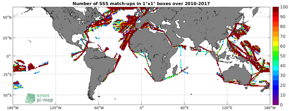
Figure 4: Number of SSS match-ups between TSG-LEGOS-DM SSS and the SMOS-L3-CATDS-CECOS-LOCEAN-V3-9DAYS-25KM SSS product for the SMOS coastal zone ( \leq 800\text{km} ) 60N-60S Pi-MEP region over 1^\circ \times 1^\circ boxes and for the full satellite product period.
