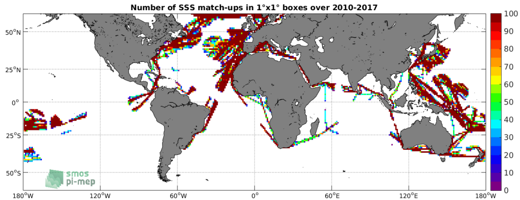
Figure 4: Number of SSS match-ups between TSG-LEGOS-DM SSS and the SMOS-L3-CATDS-CECOS-LOCEAN-V3-9DAYS-25KM SSS product for the SMOS coastal zone ( \pm 800\text{km} ) 60N-60S Pi-MEP region over 1^\circ \times 1^\circ boxes and for the full satellite product period.
