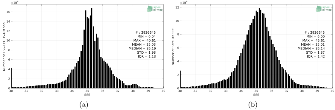
Figure 2: Histograms of SSS from TSG-LEGOS-DM (a) and SMOS-L3-CATDS-CECOS-LOCEAN-V3-9DAYS-25KM (b) considering all match-up pairs per bins of 0.1 over the SMOS coastal zone ( \approx 800 km) 60N-60S Pi-MEP region and for the full satellite product period.
