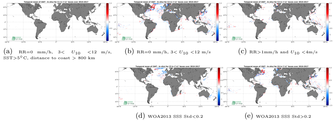
Figure 12: Temporal mean gridded over spatial boxes of size 1^\circ \times 1^\circ of \Delta SSS (SMOS-L3-CATDS-CECOS-LOCEAN-V3-9DAYS-25KM - TSG-LEGOS-DM) for 5 different subdatasets corresponding to: RR=0 mm/h, 3 < U_{10} < 12 m/s, SST > 5^\circ C , distance to coast > 800 km (a), RR=0 mm/h, 3 < U_{10} < 12 m/s (b), RR > 1 mm/h and U_{10} < 4 m/s (c), WOA2013 SSS Std < 0.2 (d), WOA2013 SSS Std > 0.2 (e).
