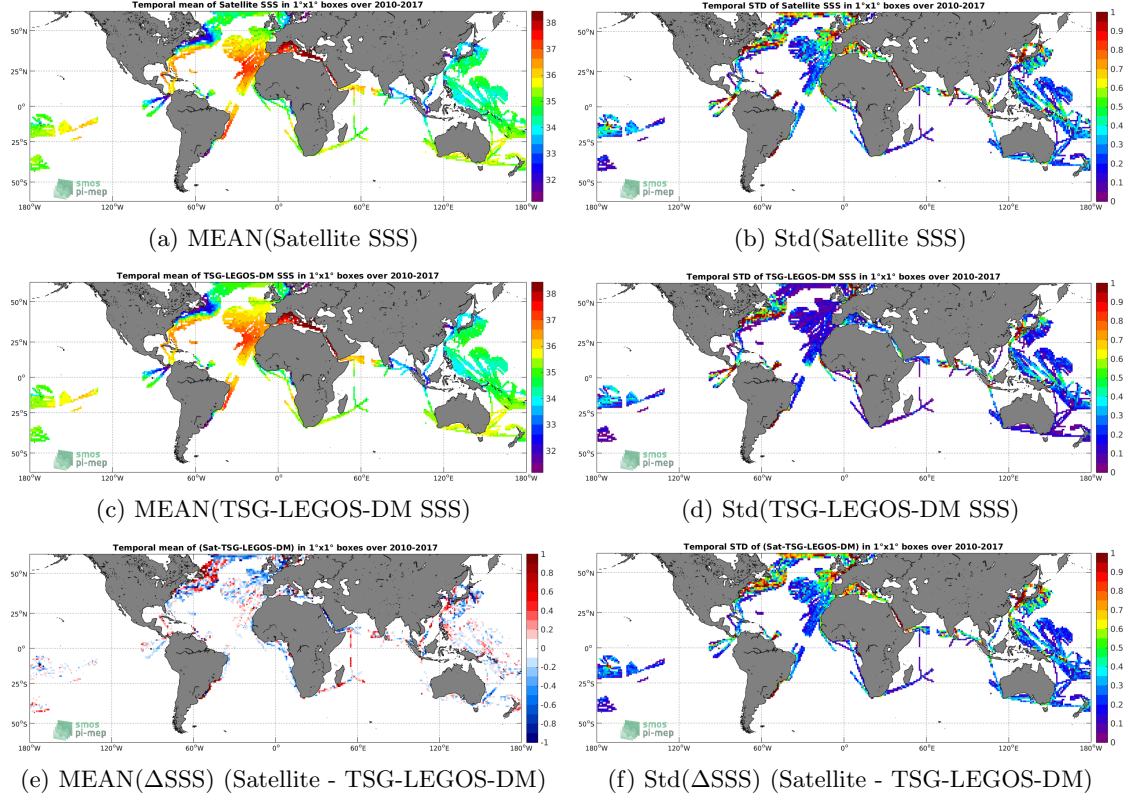
Figure 6: Temporal mean (left) and Std (right) of SSS from SMOS-L3-CATDS-CECOS-LOCEAN-V3-9DAYS-25KM (top), TSG-LEGOS-DM (middle), and of \Delta SSS (Satellite - TSG-LEGOS-DM). Only match-up pairs are used to generate these maps.
