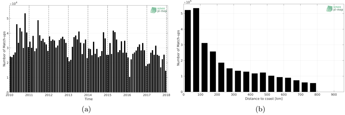
Figure 1: Number of match-ups between TSG-LEGOS-DM and SMOS-L3-CATDS-CECOS-LOCEAN-V3-9DAYS-25KM SSS as a function of time (a) and as function of the distance to coast (b) over the SMOS coastal zone ( \approx 800 km) 60N-60S Pi-MEP region and for the full satellite product period.
