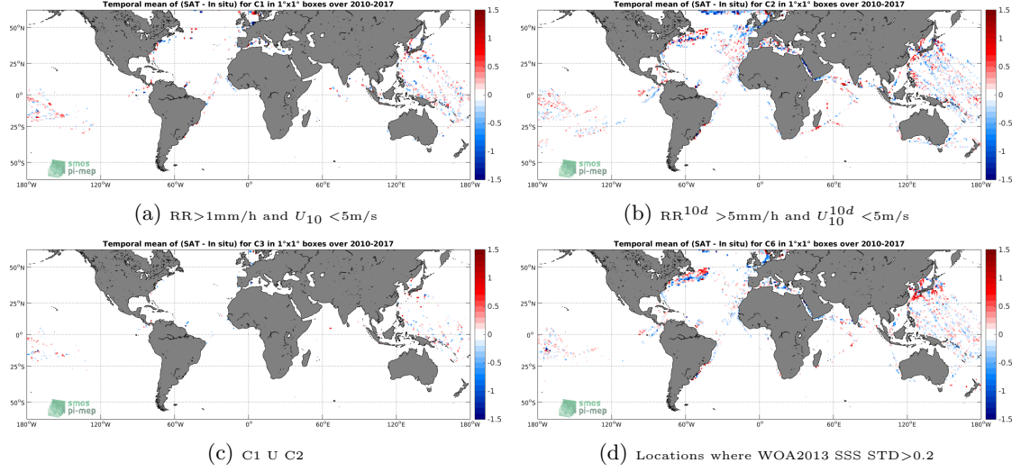
Figure 12: Temporal mean gridded over spatial boxes of size 1^\circ \times 1^\circ of \Delta SSS (SMOS-L3-CATDS-CECOS-LOCEAN-V3-9DAYS-25KM - TSG-LEGOS-DM) for 4 different subdatasets corresponding to: RR > 1\text{mm/h} and U_{10} < 5\text{m/s} (a), RR^{10d} > 5\text{mm/h} and U_{10}^{10d} < 5\text{m/s} (b), C1 U C2 (c), Locations where WOA2013 SSS STD > 0.2 (d).
