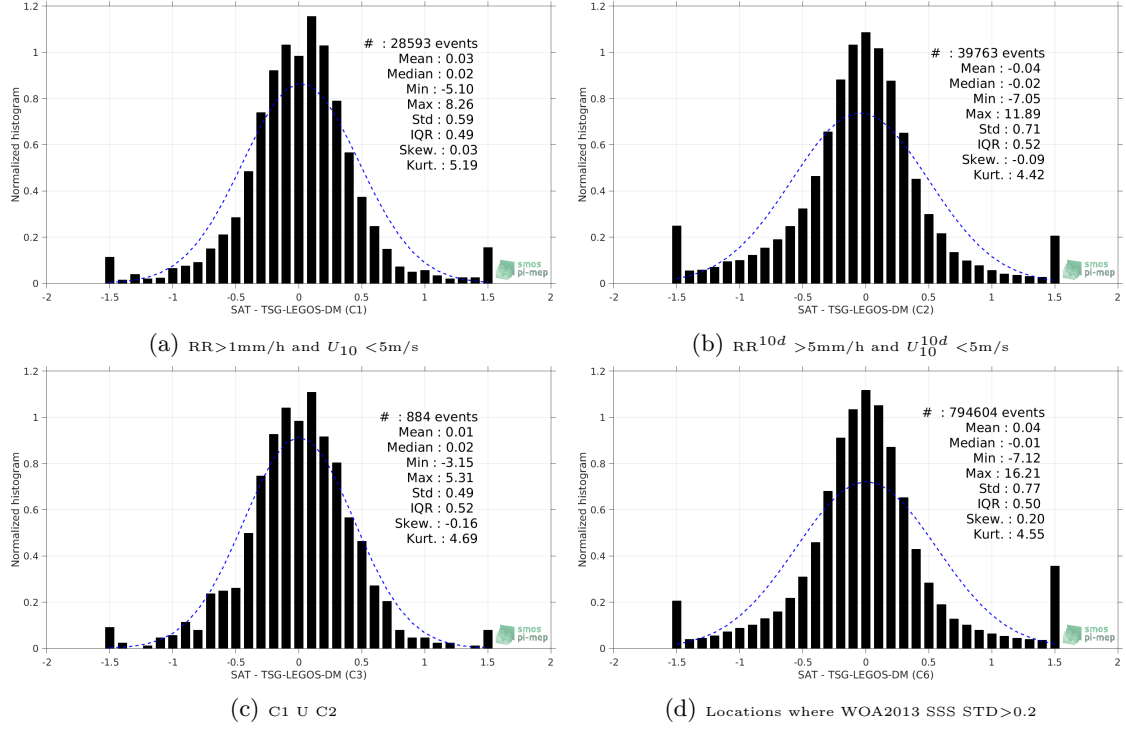
Figure 13: Normalized histogram of \Delta SSS (SMOS-L3-CATDS-CECOS-LOCEAN-V3-9DAYS-25KM - TSG-LEGOS-DM) for 6 different subdatasets corresponding to: RR > 1\text{mm/h} and U_{10} < 5\text{m/s} (a), RR^{10d} > 5\text{mm/h} and U_{10}^{10d} < 5\text{m/s} (b), C1 U C2 (c), Locations where WOA2013 SSS STD > 0.2 (d).
