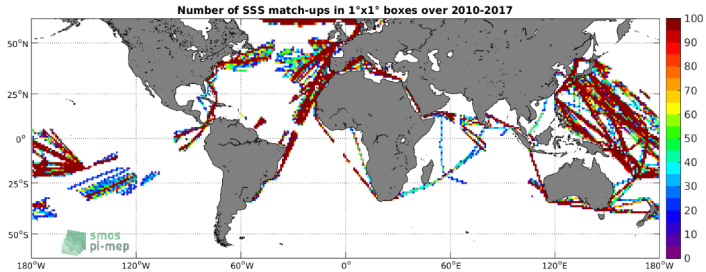
Figure 4: Number of SSS match-ups between TSG-LEGOS-DM SSS and the SMOS-L3-CATDS-CECOS-LOCEAN-V3-9DAYS-25KM SSS product for the SMOS coastal zone ( \geq 800 km) 60N-60S Pi-MEP region over 1^\circ \times 1^\circ boxes and for the full satellite product period.
