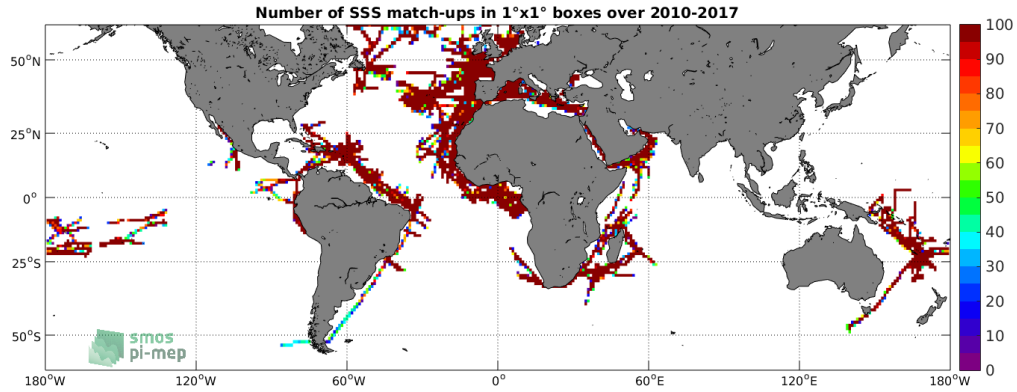
Figure 4: Number of SSS match-ups between TSG-GOSUD-Research-vessel SSS and the SMOS-L3-CATDS-CECOS-LOCEAN-V3-9DAYS-25KM SSS product for the SMOS coastal zone ( \geq 800\text{km} ) 60^\circ\text{N} - 60^\circ\text{S} Pi-MEP region over 1^\circ \times 1^\circ boxes and for the full satellite product period.
