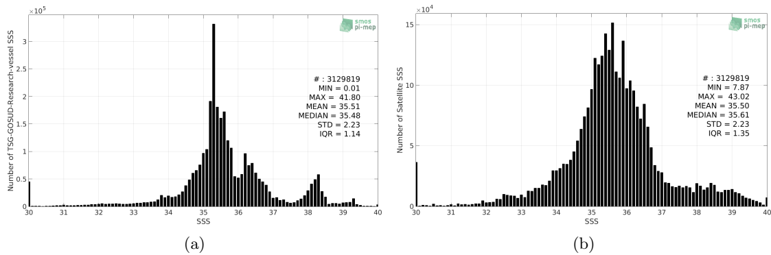
Figure 2: Histograms of SSS from TSG-GOSUD-Research-vessel (a) and SMOS-L3-CATDS-CECOS-LOCEAN-V3-9DAYS-25KM (b) considering all match-up pairs per bins of 0.1 over the SMOS coastal zone ( \geq 800\text{km} ) 60N-60S Pi-MEP region and for the full satellite product period.
