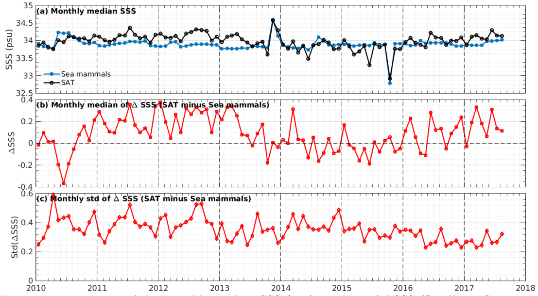
Figure 7: Time series of the monthly median SSS (top), median of \Delta\text{SSS} (Satellite - Sea mammals) and Std of \Delta\text{SSS} (Satellite - Sea mammals) over the SMOS coastal zone ( \pm 800\text{km} 60\text{N} - 60\text{S} Pi-MEP region considering all match-ups collected by the Pi-MEP.
