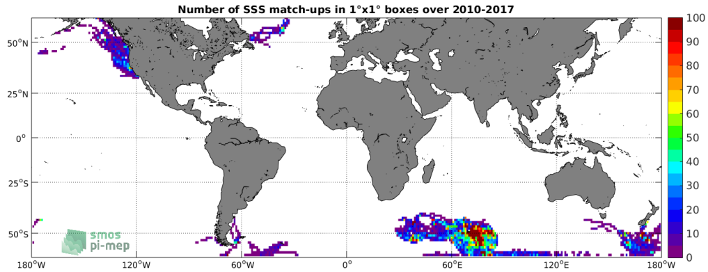
Figure 4: Number of SSS match-ups between Sea mammals SSS and the SMOS-L3-CATDS-CECOS-LOCEAN-V3-9DAYS-25KM SSS product for the SMOS coastal zone ( \geq 800 km) 60N-60S Pi-MEP region over 1^\circ \times 1^\circ boxes and for the full satellite product period.
