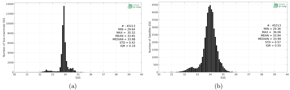
Figure 2: Histograms of SSS from Sea mammals (a) and SMOS-L3-CATDS-CECOS-LOCEAN-V3-9DAYS-25KM (b) considering all match-up pairs per bins of 0.1 over the SMOS coastal zone ( \leq 800 km) 60N-60S Pi-MEP region and for the full satellite product period.
