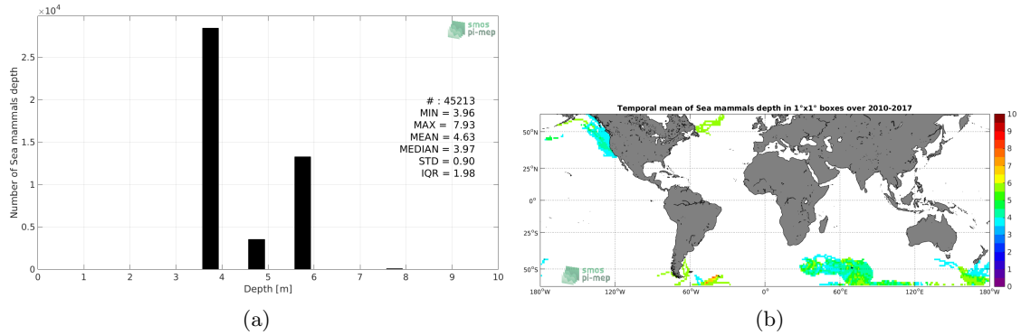
Figure 3: Histograms of the depth of the upper level SSS measurements from Sea mammals in the Match-up DataBase for the SMOS coastal zone ( \geq 800\text{km} ) 60N-60S Pi-MEP region (a) and temporal mean spatial distribution of pressure of the in situ SSS data over 1^\circ \times 1^\circ boxes and for the full satellite product period (b).
