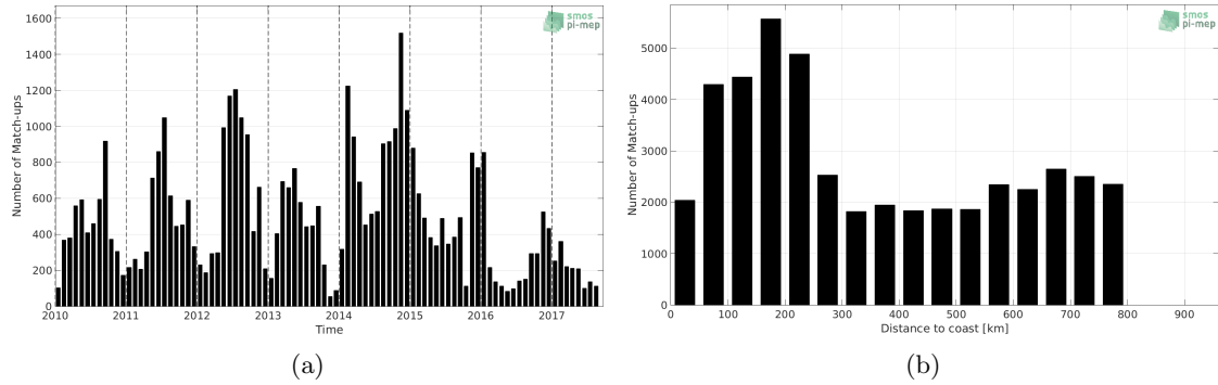
Figure 1: Number of match-ups between Sea mammals and SMOS-L3-CATDS-CECOS-LOCEAN-V3-9DAYS-25KM SSS as a function of time (a) and as function of the distance to coast (b) over the SMOS coastal zone ( \leq 800 km) 60N-60S Pi-MEP region and for the full satellite product period.
