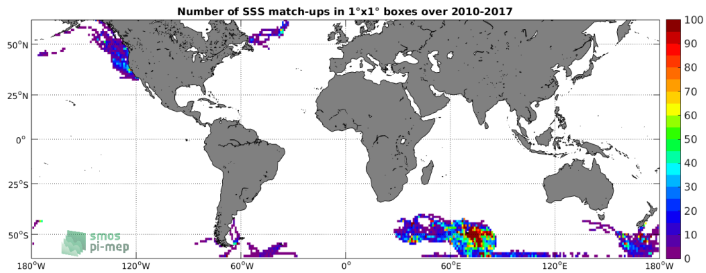
Figure 4: Number of SSS match-ups between Sea mammals SSS and the SMOS-L3-CATDS-CECOS-LOCEAN-V3-9DAYS-25KM SSS product for the SMOS coastal zone ( \geq 800\text{km} ) 60N-60S Pi-MEP region over 1^\circ \times 1^\circ boxes and for the full satellite product period.
