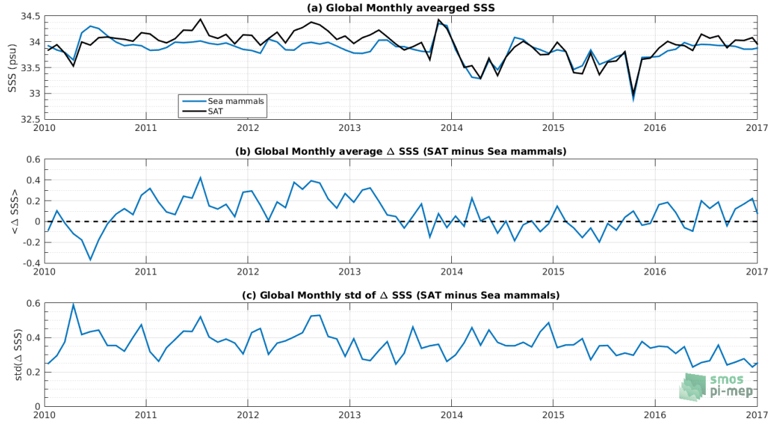
Figure 7: Time series of the monthly averaged mean SSS (top), mean \Delta SSS (Satellite - Sea mammals) and Std of \Delta SSS (Satellite - Sea mammals) over the SMOS coastal zone ( \geq 800 km) 60N-60S Pi-MEP region considering all match-ups collected by the Pi-MEP platform.
