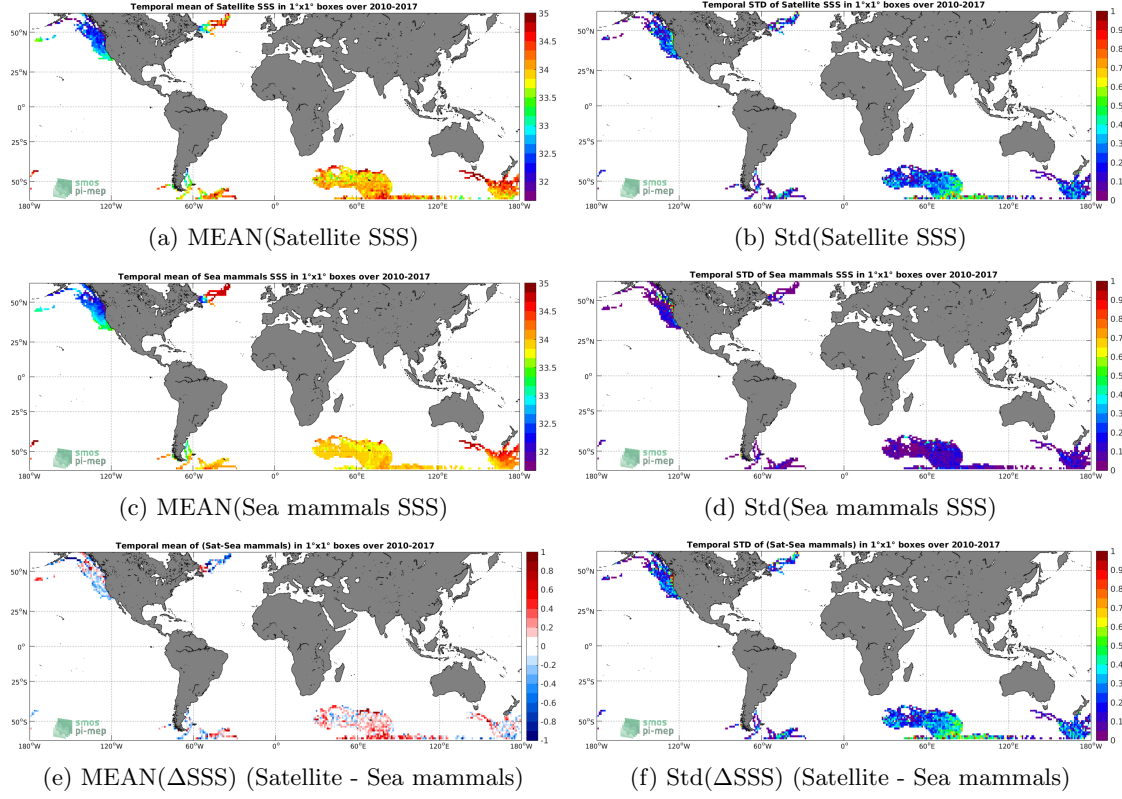
Figure 6: Temporal mean (left) and Std (right) of SSS from SMOS-L3-CATDS-CECOS-LOCEAN-V3-9DAYS-25KM (top), Sea mammals (middle), and of \Delta SSS (Satellite - Sea mammals). Only match-up pairs are used to generate these maps.
