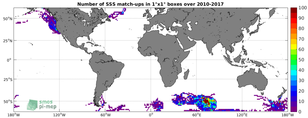
Figure 4: Number of SSS match-ups between Sea mammals SSS and the SMOS-L3-CATDS-CECOS-LOCEAN-V3-9DAYS-25KM SSS product for the SMOS coastal zone ( \pm 800\text{km} ) 60N-60S Pi-MEP region over 1^\circ \times 1^\circ boxes and for the full satellite product period.
