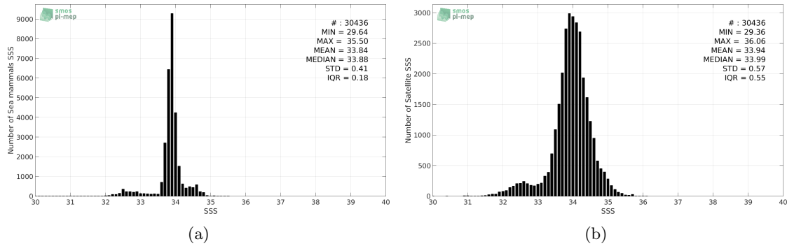
Figure 2: Histograms of SSS from Sea mammals (a) and SMOS-L3-CATDS-CECOS-LOCEAN-V3-9DAYS-25KM (b) considering all match-up pairs per bins of 0.1 over the SMOS coastal zone ( \geq 800 km) 60N-60S Pi-MEP region and for the full satellite product period.
