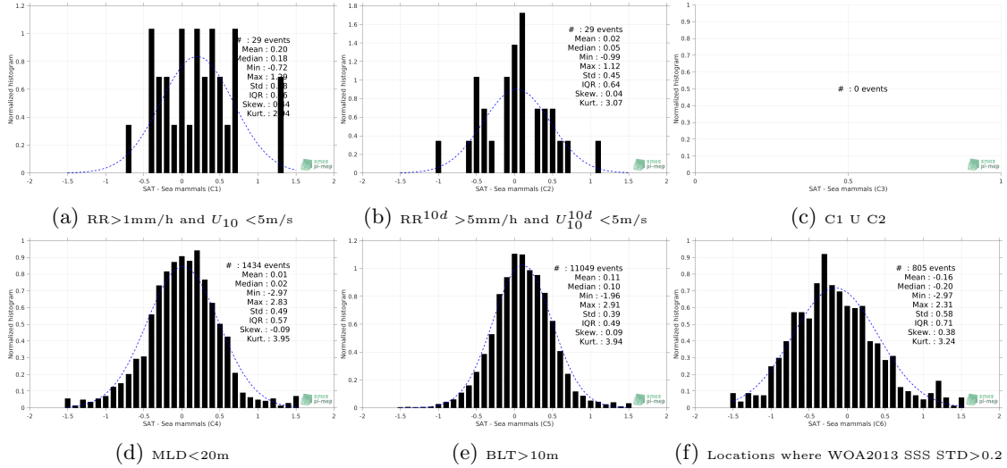
Figure 13: Normalized histogram of \Delta SSS (SMOS-L3-CATDS-CECOS-LOCEAN-V3-9DAYS-25KM - Sea mammals) for 6 different subdatasets corresponding to: RR > 1\text{mm/h} and U_{10} < 5\text{m/s} (a), RR^{10d} > 5\text{mm/h} and U_{10}^{10d} < 5\text{m/s} (b), C1 U C2 (c), MLD < 20\text{m} (d), BLT > 10\text{m} (e), Locations where WOA2013 SSS STD > 0.2 (f).
