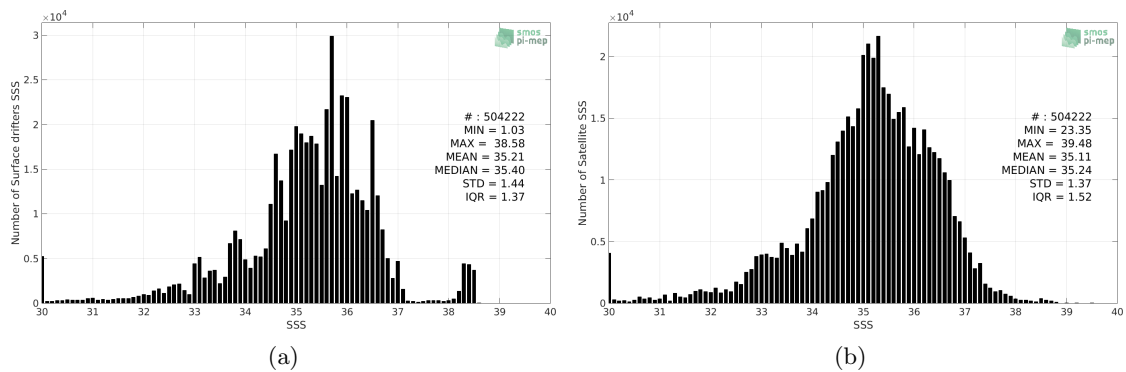
Figure 2: Histograms of SSS from Surface drifters (a) and SMOS-L3-CATDS-CECOS-LOCEAN-V3-9DAYS-25KM (b) considering all match-up pairs per bins of 0.1 over the SMOS coastal zone ( \approx 800\text{km} ) 60N-60S Pi-MEP region and for the full satellite product period.
