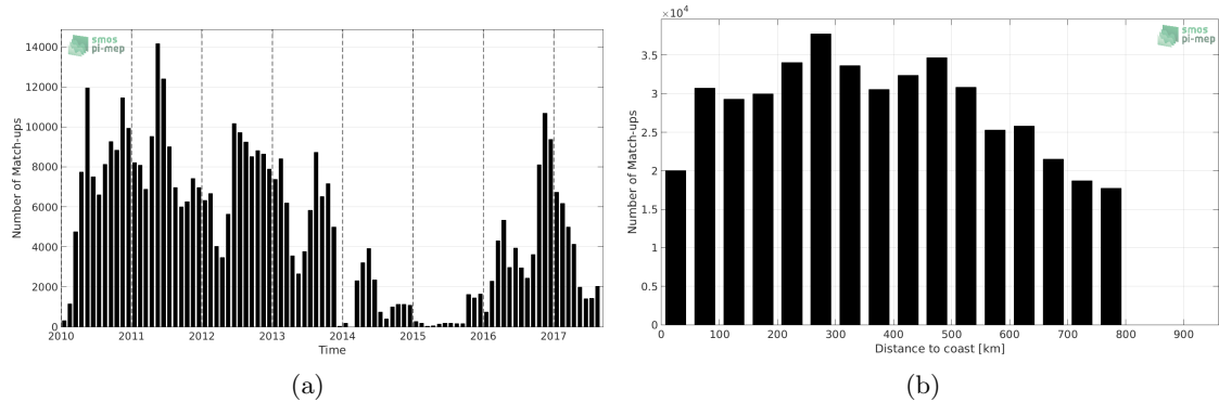
Figure 1: Number of match-ups between Surface drifters and SMOS-L3-CATDS-CECOS-LOCEAN-V3-9DAYS-25KM SSS as a function of time (a) and as function of the distance to coast (b) over the SMOS coastal zone ( \approx 800 km) 60N-60S Pi-MEP region and for the full satellite product period.
