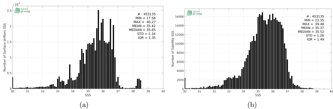
Figure 2: Histograms of SSS from Surface drifters (a) and SMOS-L3-CATDS-CECOS-LOCEAN-V3-9DAYS-25KM (b) considering all match-up pairs per bins of 0.1 over the SMOS coastal zone ( \approx 800 km) 60N-60S Pi-MEP region and for the full satellite product period.
