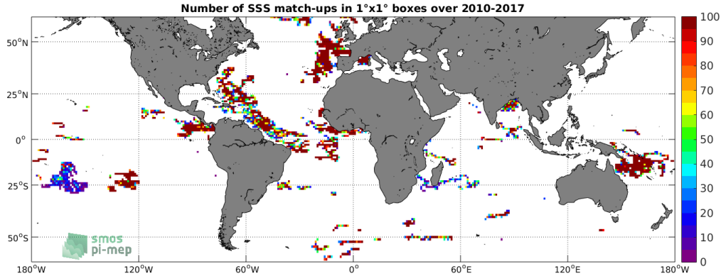
Figure 3: Number of SSS match-ups between Surface drifters SSS and the SMOS-L3-CATDS-CECOS-LOCEAN-V3-9DAYS-25KM SSS product for the SMOS coastal zone ( \approx 800\text{km} ) 60N-60S Pi-MEP region over 1°x1° boxes and for the full satellite product period.
