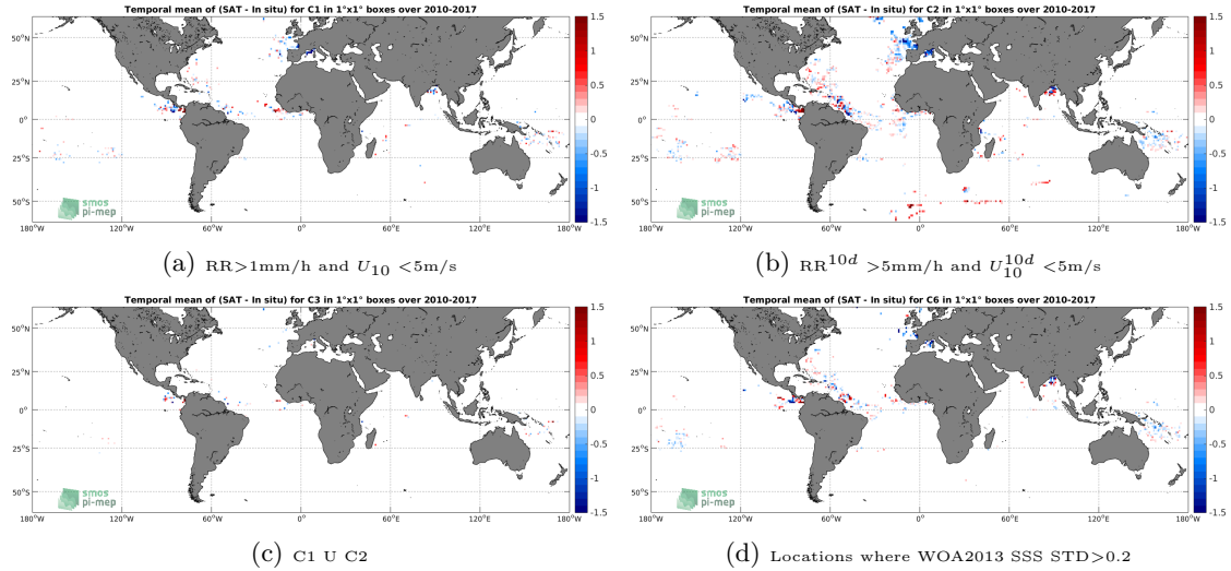
Figure 11: Temporal mean gridded over spatial boxes of size 1^\circ \times 1^\circ of \Delta SSS (SMOS-L3-CATDS-CECOS-LOCEAN-V3-9DAYS-25KM - Surface drifters) for 4 different subdatasets corresponding to: RR > 1\text{mm/h} and U_{10} < 5\text{m/s} (a), RR^{10d} > 5\text{mm/h} and U_{10}^{10d} < 5\text{m/s} (b), C1 U C2 (c), Locations where WOA2013 SSS STD > 0.2 (d).
