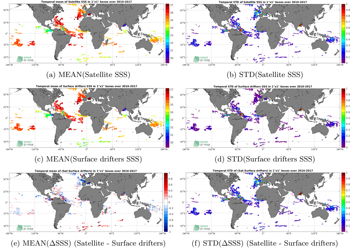
Figure 5: Temporal mean (left) and STD (right) of SSS from SMOS-L3-CATDS-CECOS-LOCEAN-V3-9DAYS-25KM (top), Surface drifters (middle), and of \Delta SSS (Satellite - Surface drifters). Only match-up pairs are used to generate these maps.
