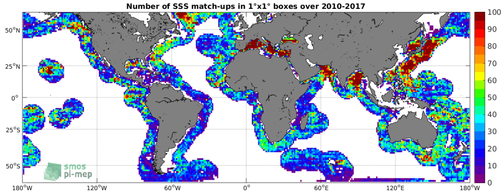
Figure 4: Number of SSS match-ups between Argo SSS and the SMOS-L3-CATDS-CECOS-LOCEAN-V3-9DAYS-25KM SSS product for the SMOS coastal zone ( \geq 800\text{km} ) 60N-60S Pi-MEP region over 1^\circ \times 1^\circ boxes and for the full satellite product period.
