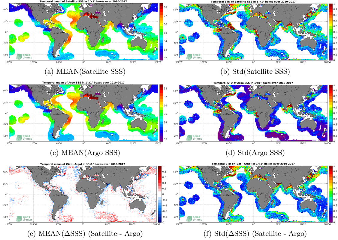
Figure 6: Temporal mean (left) and Std (right) of SSS from SMOS-L3-CATDS-CECOS-LOCEAN-V3-9DAYS-25KM (top), Argo (middle), and of \Delta SSS (Satellite - Argo). Only match-up pairs are used to generate these maps.
