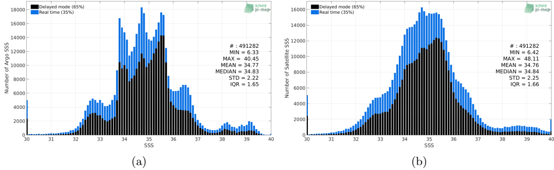
Figure 2: Histograms of SSS from Argo (a) and SMOS-L3-CATDS-CECOS-LOCEAN-V3-9DAYS-25KM (b) considering all match-up pairs per bins of 0.1 over the SMOS coastal zone ( \pm 800 km) 60N-60S Pi-MEP region and for the full satellite product period.
