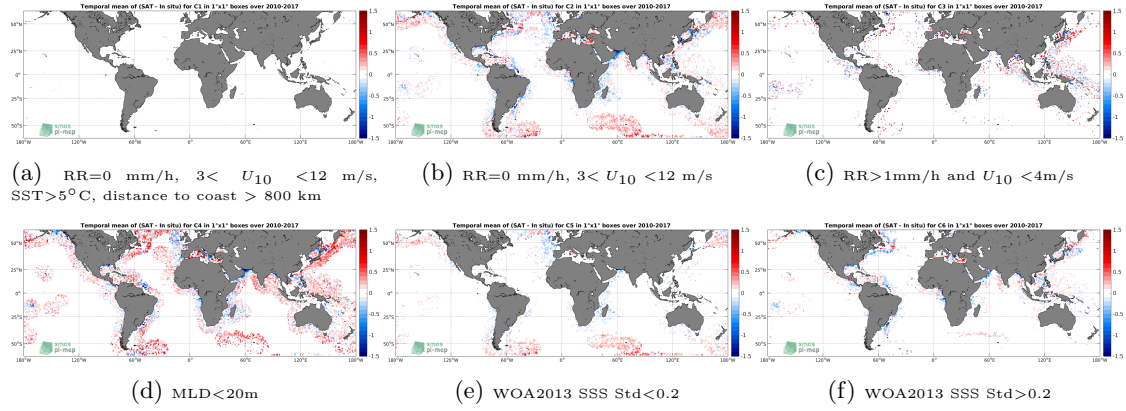
Figure 12: Temporal mean gridded over spatial boxes of size 1^\circ \times 1^\circ of \Delta SSS (SMOS-L3-CATDS-CECOS-LOCEAN-V3-9DAYS-25KM - Argo) for 6 different subdatasets corresponding to: RR=0 mm/h, 3 < U_{10} < 12 m/s, SST > 5^\circ C , distance to coast > 800 km (a), RR=0 mm/h, 3 < U_{10} < 12 m/s (b), RR > 1 mm/h and U_{10} < 4 m/s (c), MLD < 20 m (d), WOA2013 SSS Std < 0.2 (e), WOA2013 SSS Std > 0.2 (f).
