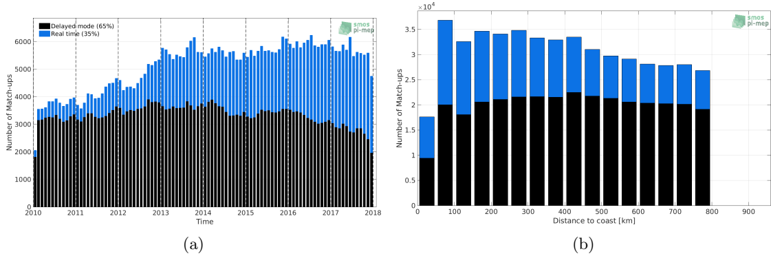
Figure 1: Number of match-ups between Argo and SMOS-L3-CATDS-CECOS-LOCEAN-V3-9DAYS-25KM SSS as a function of time (a) and as function of the distance to coast (b) over the SMOS coastal zone ( \pm 800 km) 60N-60S Pi-MEP region and for the full satellite product period.
