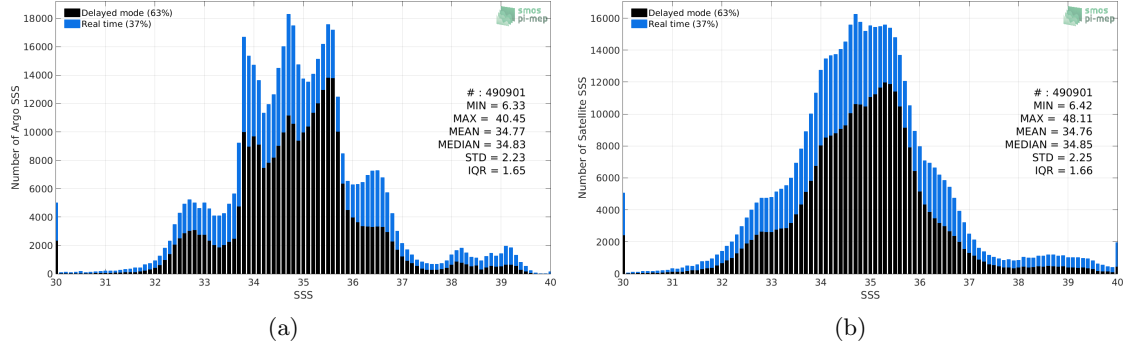
Figure 2: Histograms of SSS from Argo (a) and SMOS-L3-CATDS-CECOS-LOCEAN-V3-9DAYS-25KM (b) considering all match-up pairs per bins of 0.1 over the SMOS coastal zone ( \geq 800\text{km} ) 60N-60S Pi-MEP region and for the full satellite product period.
