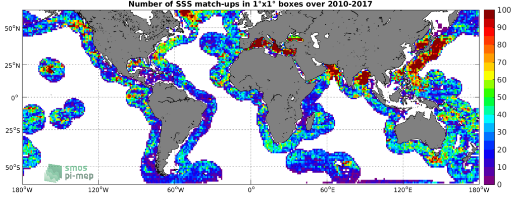
Figure 4: Number of SSS match-ups between Argo SSS and the SMOS-L3-CATDS-CECOS-LOCEAN-V3-9DAYS-25KM SSS product for the SMOS coastal zone ( \pm 800\text{km} ) 60N-60S Pi-MEP region over 1^\circ \times 1^\circ boxes and for the full satellite product period.
