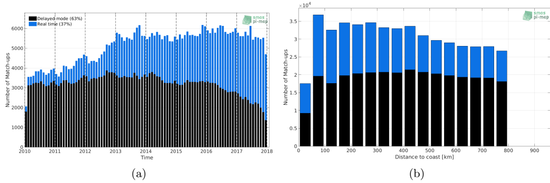
Figure 1: Number of match-ups between Argo and SMOS-L3-CATDS-CECOS-LOCEAN-V3-9DAYS-25KM SSS as a function of time (a) and as function of the distance to coast (b) over the SMOS coastal zone ( \leq 800\text{km} ) 60N-60S Pi-MEP region and for the full satellite product period.
