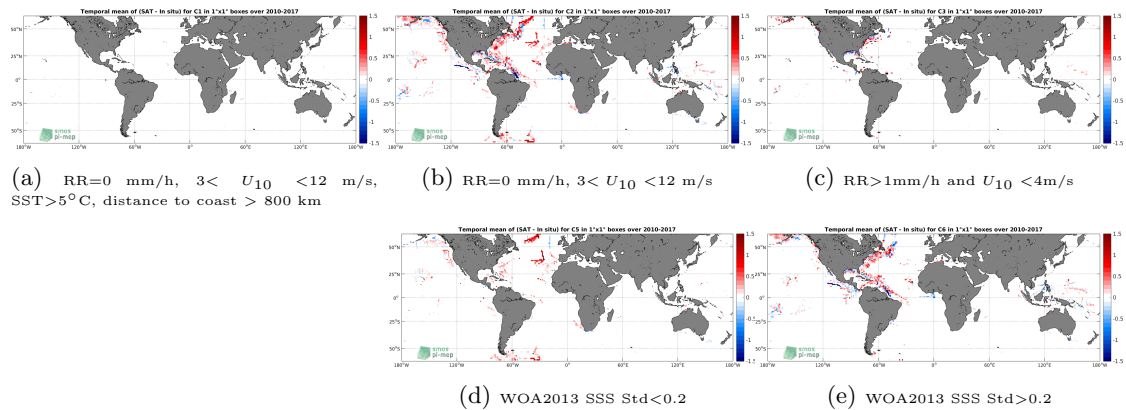
Figure 12: Temporal mean gridded over spatial boxes of size 1^\circ \times 1^\circ of \Delta SSS (SMOS-L3-CATDS-CECOS-LOCEAN-V3-18DAYS-25KM - TSG-SAMOS) for 5 different subdatasets corresponding to:RR=0 mm/h, 3 < U_{10} < 12 m/s, SST >5^\circ C, distance to coast > 800 km (a), RR=0 mm/h, 3 < U_{10} < 12 m/s (b), RR >1 mm/h and U_{10} < 4 m/s (c), WOA2013 SSS Std <0.2 (d), WOA2013 SSS Std >0.2 (e).
