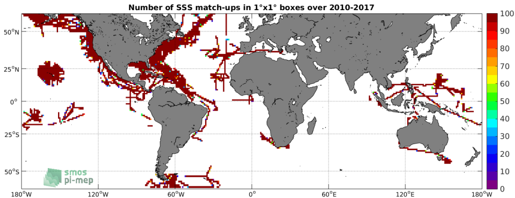
Figure 4: Number of SSS match-ups between TSG-SAMOS SSS and the SMOS-L3-CATDS-CECOS-LOCEAN-V3-18DAYS-25KM SSS product for the SMOS coastal zone ( \approx 800\text{km} ) 60N-60S Pi-MEP region over 1^\circ \times 1^\circ boxes and for the full satellite product period.
