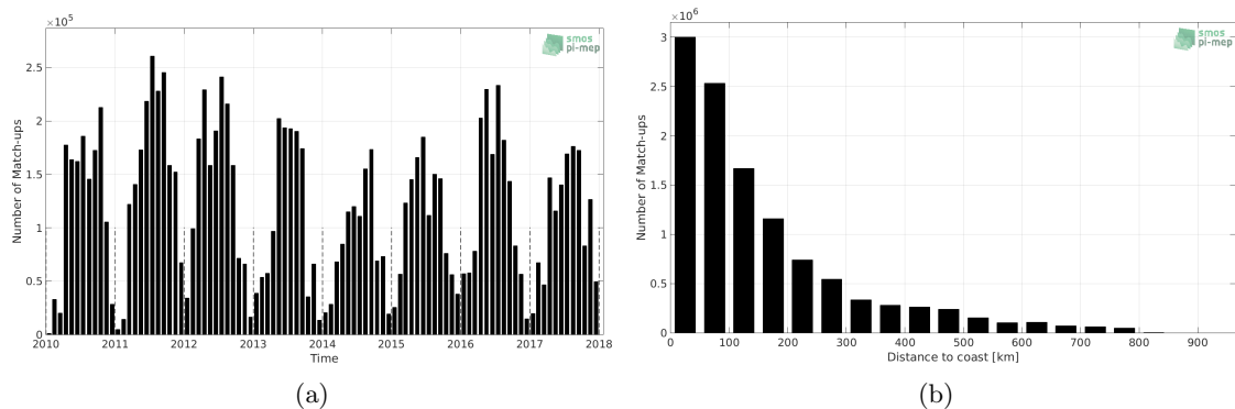
Figure 1: Number of match-ups between TSG-SAMOS and SMOS-L3-CATDS-CECOS-LOCEAN-V3-18DAYS-25KM SSS as a function of time (a) and as function of the distance to coast (b) over the SMOS coastal zone ( \approx 800\text{km} ) 60N-60S Pi-MEP region and for the full satellite product period.
