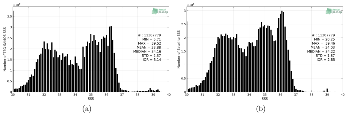
Figure 2: Histograms of SSS from TSG-SAMOS (a) and SMOS-L3-CATDS-CECOS-LOCEAN-V3-18DAYS-25KM (b) considering all match-up pairs per bins of 0.1 over the SMOS coastal zone ( \approx 800\text{km} ) 60N-60S Pi-MEP region and for the full satellite product period.
