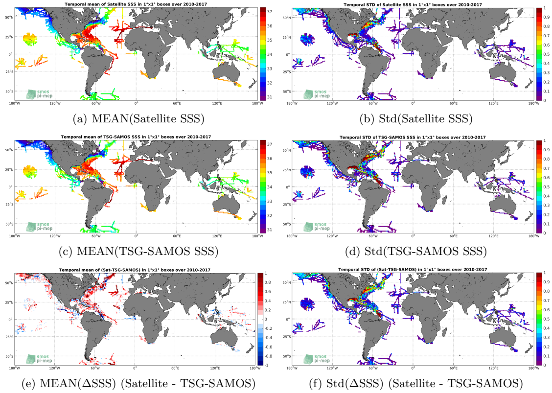
Figure 6: Temporal mean (left) and Std (right) of SSS from SMOS-L3-CATDS-CECOS-LOCEAN-V3-18DAYS-25KM (top), TSG-SAMOS (middle), and of \Delta SSS (Satellite - TSG-SAMOS). Only match-up pairs are used to generate these maps.
