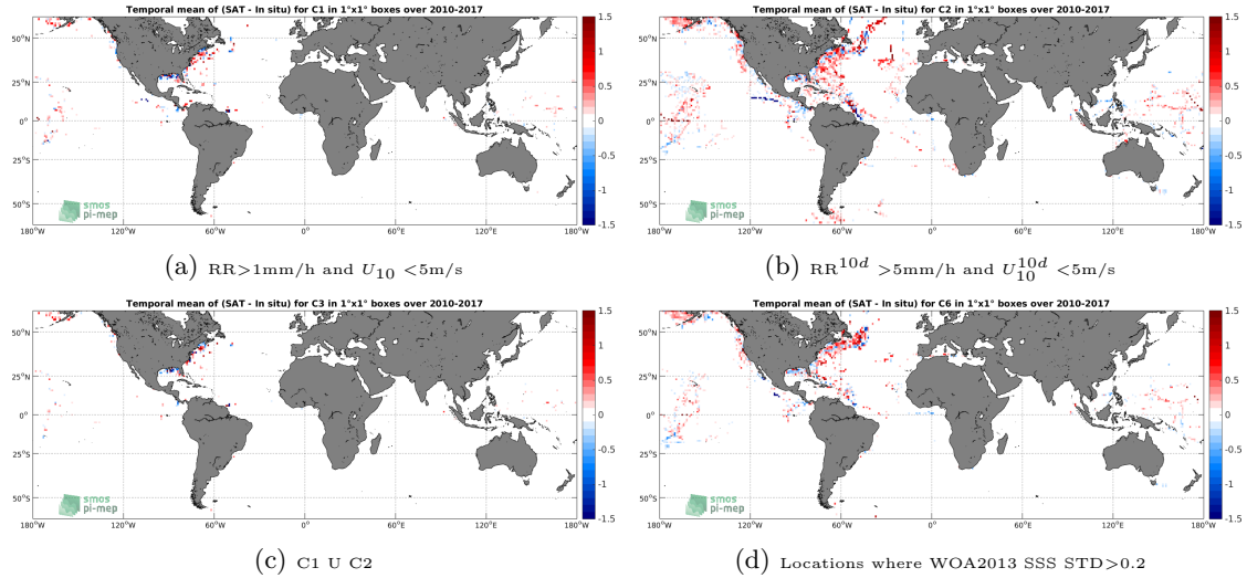
Figure 12: Temporal mean gridded over spatial boxes of size 1^\circ \times 1^\circ of \Delta SSS (SMOS-L3-CATDS-CECOS-LOCEAN-V3-18DAYS-25KM - TSG-SAMOS) for 4 different subdatasets corresponding to: RR > 1\text{mm/h} and U_{10} < 5\text{m/s} (a), RR^{10d} > 5\text{mm/h} and U_{10}^{10d} < 5\text{m/s} (b), C1 U C2 (c), Locations where WOA2013 SSS STD > 0.2 (d).
