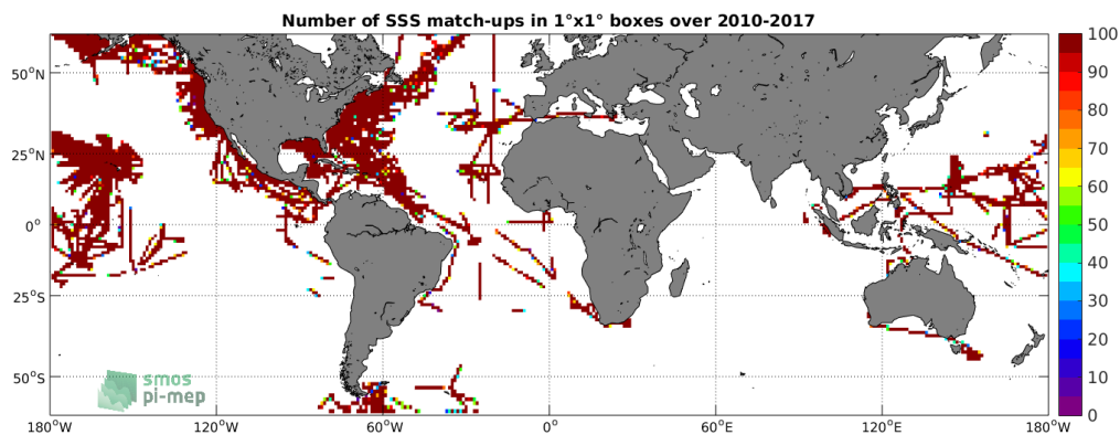
Figure 4: Number of SSS match-ups between TSG-SAMOS SSS and the SMOS-L3-CATDS-CECOS-LOCEAN-V3-18DAYS-25KM SSS product for the SMOS coastal zone ( \pm 800\text{km} ) 60N-60S Pi-MEP region over 1^\circ \times 1^\circ boxes and for the full satellite product period.
