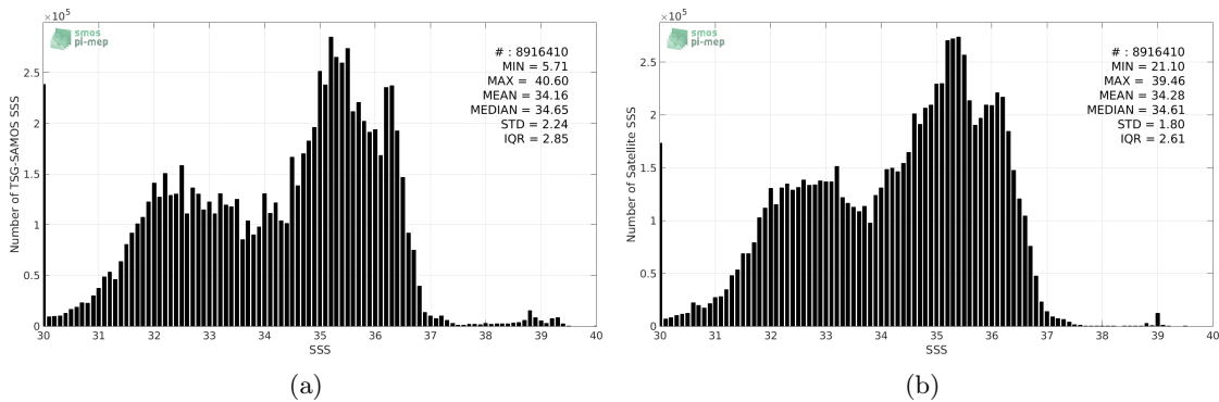
Figure 2: Histograms of SSS from TSG-SAMOS (a) and SMOS-L3-CATDS-CECOS-LOCEAN-V3-18DAYS-25KM (b) considering all match-up pairs per bins of 0.1 over the SMOS coastal zone ( \approx 800 km) 60N-60S Pi-MEP region and for the full satellite product period.
