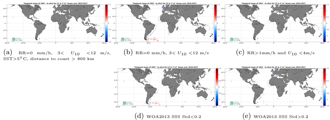
Figure 12: Temporal mean gridded over spatial boxes of size 1^\circ \times 1^\circ of \Delta SSS (SMOS-L3-CATDS-CECOS-LOCEAN-V3-18DAYS-25KM - TSG-POLARSTERN) for 5 different subdatasets corresponding to:RR=0 mm/h, 3 < U_{10} < 12 m/s, SST >5^\circ C, distance to coast > 800 km (a), RR=0 mm/h, 3 < U_{10} < 12 m/s (b), RR >1 mm/h and U_{10} < 4 m/s (c), WOA2013 SSS Std <0.2 (d), WOA2013 SSS Std >0.2 (e).
