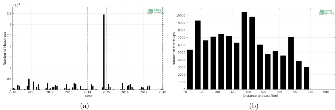
Figure 1: Number of match-ups between TSG-POLARSTERN and SMOS-L3-CATDS-CECOS-LOCEAN-V3-18DAYS-25KM SSS as a function of time (a) and as function of the distance to coast (b) over the SMOS coastal zone ( \approx 800 km) 60N-60S Pi-MEP region and for the full satellite product period.
