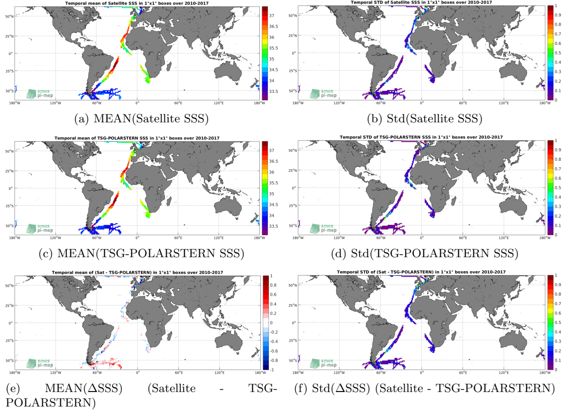
Figure 6: Temporal mean (left) and Std (right) of SSS from SMOS-L3-CATDS-CECOS-LOCEAN-V3-18DAYS-25KM (top), TSG-POLARSTERN (middle), and of \Delta SSS (Satellite - TSG-POLARSTERN). Only match-up pairs are used to generate these maps.
