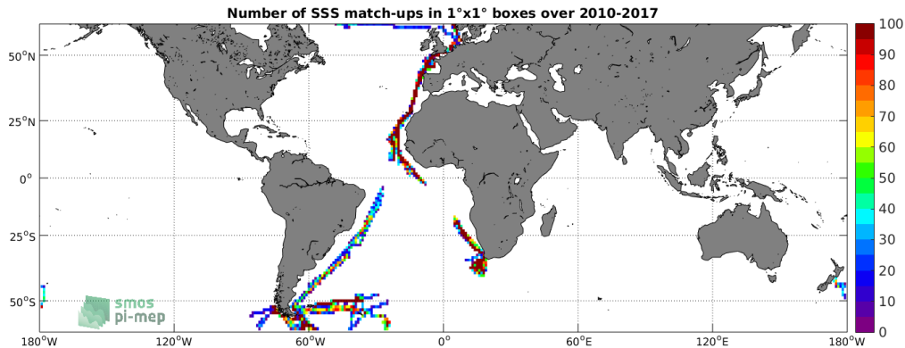
Figure 4: Number of SSS match-ups between TSG-POLARSTERN SSS and the SMOS-L3-CATDS-CECOS-LOCEAN-V3-18DAYS-25KM SSS product for the SMOS coastal zone ( \approx 800\text{km} ) 60N-60S Pi-MEP region over 1^\circ \times 1^\circ boxes and for the full satellite product period.
