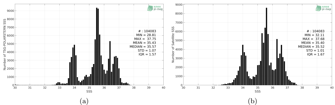
Figure 2: Histograms of SSS from TSG-POLARSTERN (a) and SMOS-L3-CATDS-CECOS-LOCEAN-V3-18DAYS-25KM (b) considering all match-up pairs per bins of 0.1 over the SMOS coastal zone ( \approx 800 km) 60N-60S Pi-MEP region and for the full satellite product period.
