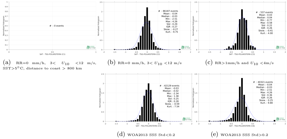
Figure 13: Normalized histogram of \Delta SSS (SMOS-L3-CATDS-CECOS-LOCEAN-V3-18DAYS-25KM - TSG-POLARSTERN) for 5 different subdatasets corresponding to: RR=0 mm/h, 3 < U_{10} < 12 m/s, SST > 5°C, distance to coast > 800 km (a), RR=0 mm/h, 3 < U_{10} < 12 m/s (b), RR > 1mm/h and U_{10} < 4 m/s (c), WOA2013 SSS Std < 0.2 (d), WOA2013 SSS Std > 0.2 (e).
