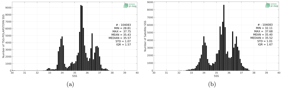
Figure 2: Histograms of SSS from TSG-POLARSTERN (a) and SMOS-L3-CATDS-CECOS-LOCEAN-V3-18DAYS-25KM (b) considering all match-up pairs per bins of 0.1 over the SMOS coastal zone ( \geq 800\text{km} ) 60N-60S Pi-MEP region and for the full satellite product period.
