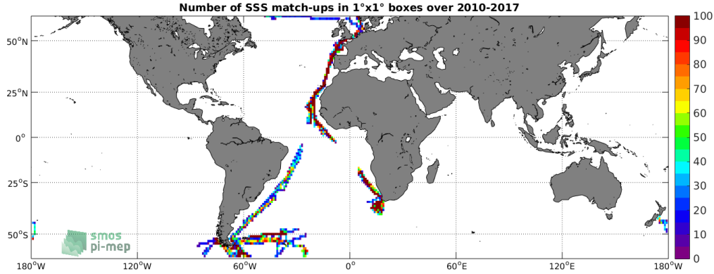
Figure 4: Number of SSS match-ups between TSG-POLARSTERN SSS and the SMOS-L3-CATDS-CECOS-LOCEAN-V3-18DAYS-25KM SSS product for the SMOS coastal zone ( \leq 800\text{km} ) 60N-60S Pi-MEP region over 1^\circ \times 1^\circ boxes and for the full satellite product period.
