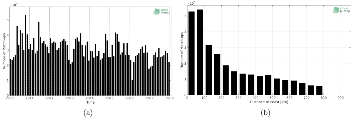
Figure 1: Number of match-ups between TSG-LEGOS-DM and SMOS-L3-CATDS-CECOS-LOCEAN-V3-18DAYS-25KM SSS as a function of time (a) and as function of the distance to coast (b) over the SMOS coastal zone ( \approx 800\text{km} ) 60N-60S Pi-MEP region and for the full satellite product period.
