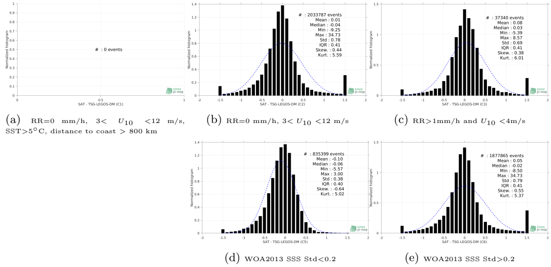
Figure 13: Normalized histogram of \Delta SSS (SMOS-L3-CATDS-CECOS-LOCEAN-V3-18DAYS-25KM - TSG-LEGOS-DM) for 5 different subdatasets corresponding to: RR=0 mm/h, 3 < U_{10} < 12 m/s, SST>5°C, distance to coast > 800 km (a), RR=0 mm/h, 3 < U_{10} < 12 m/s (b), RR>1mm/h and U_{10} < 4 m/s (c), WOA2013 SSS Std<0.2 (d), WOA2013 SSS Std>0.2 (e).
