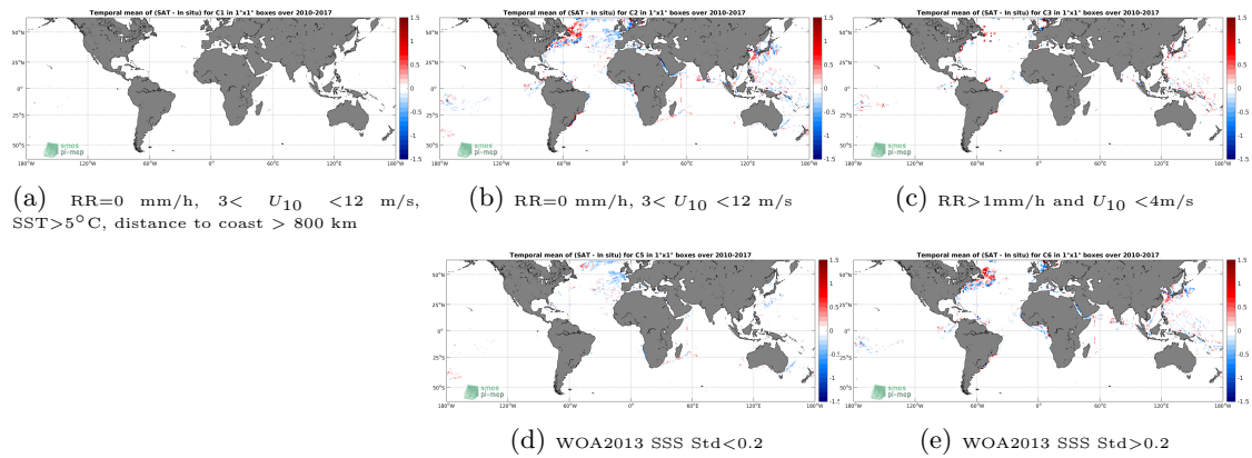
Figure 12: Temporal mean gridded over spatial boxes of size 1^\circ \times 1^\circ of \Delta SSS (SMOS-L3-CATDS-CECOS-LOCEAN-V3-18DAYS-25KM - TSG-LEGOS-DM) for 5 different subdatasets corresponding to:RR=0 mm/h, 3 < U_{10} < 12 m/s, SST >5^\circ C, distance to coast > 800 km (a), RR=0 mm/h, 3 < U_{10} < 12 m/s (b), RR >1 mm/h and U_{10} < 4 m/s (c), WOA2013 SSS Std <0.2 (d), WOA2013 SSS Std >0.2 (e).
