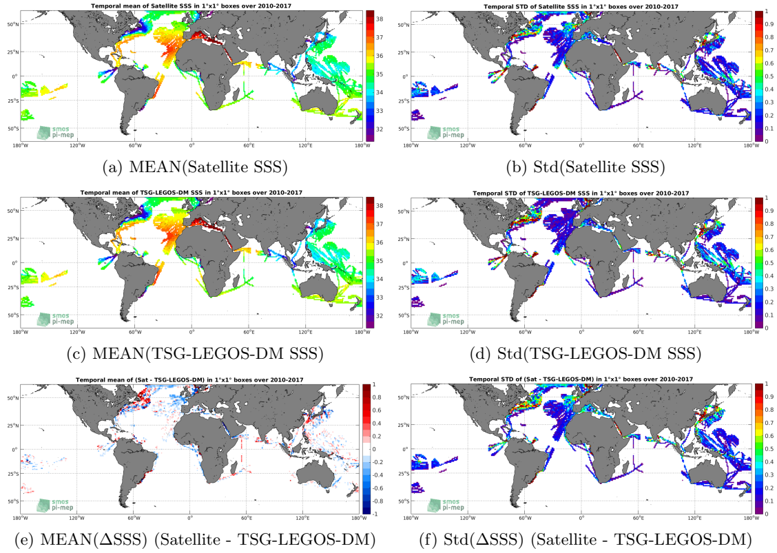
Figure 6: Temporal mean (left) and Std (right) of SSS from SMOS-L3-CATDS-CECOS-LOCEAN-V3-18DAYS-25KM (top), TSG-LEGOS-DM (middle), and of \Delta SSS (Satellite - TSG-LEGOS-DM). Only match-up pairs are used to generate these maps.
