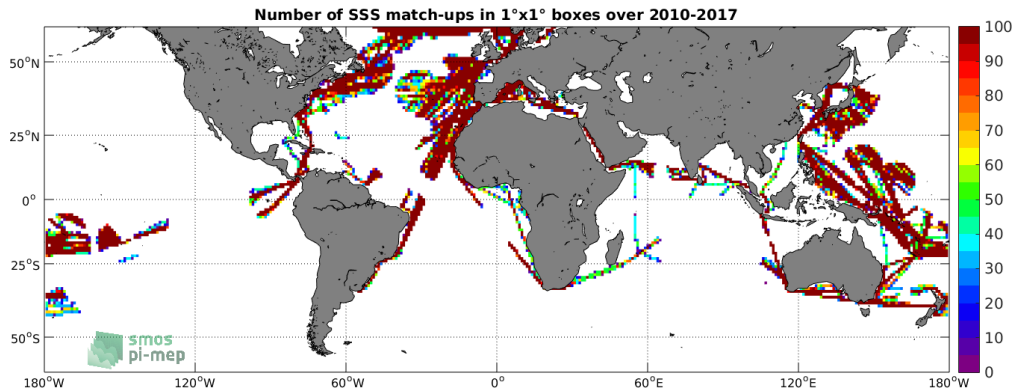
Figure 4: Number of SSS match-ups between TSG-LEGOS-DM SSS and the SMOS-L3-CATDS-CECOS-LOCEAN-V3-18DAYS-25KM SSS product for the SMOS coastal zone ( \geq 800\text{km} ) 60N-60S Pi-MEP region over 1^\circ \times 1^\circ boxes and for the full satellite product period.
