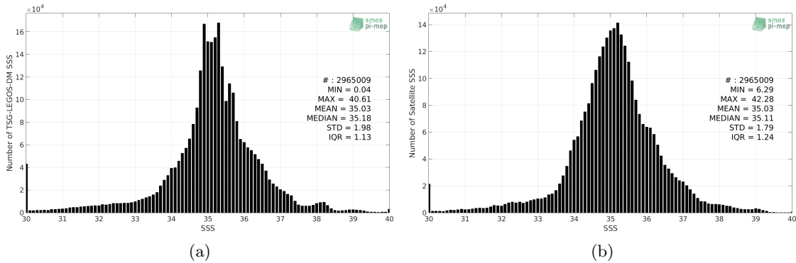
Figure 2: Histograms of SSS from TSG-LEGOS-DM (a) and SMOS-L3-CATDS-CECOS-LOCEAN-V3-18DAYS-25KM (b) considering all match-up pairs per bins of 0.1 over the SMOS coastal zone ( \approx 800\text{km} ) 60N-60S Pi-MEP region and for the full satellite product period.
