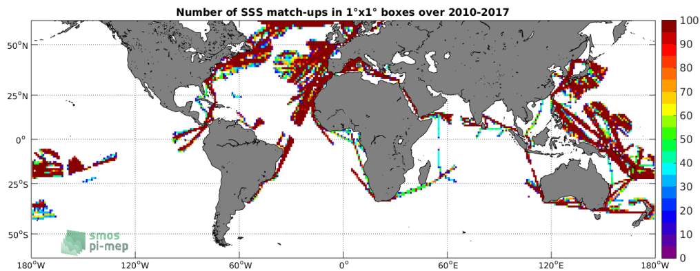
Figure 4: Number of SSS match-ups between TSG-LEGOS-DM SSS and the SMOS-L3-CATDS-CECOS-LOCEAN-V3-18DAYS-25KM SSS product for the SMOS coastal zone ( \pm 800\text{km} ) 60N-60S Pi-MEP region over 1^\circ \times 1^\circ boxes and for the full satellite product period.
