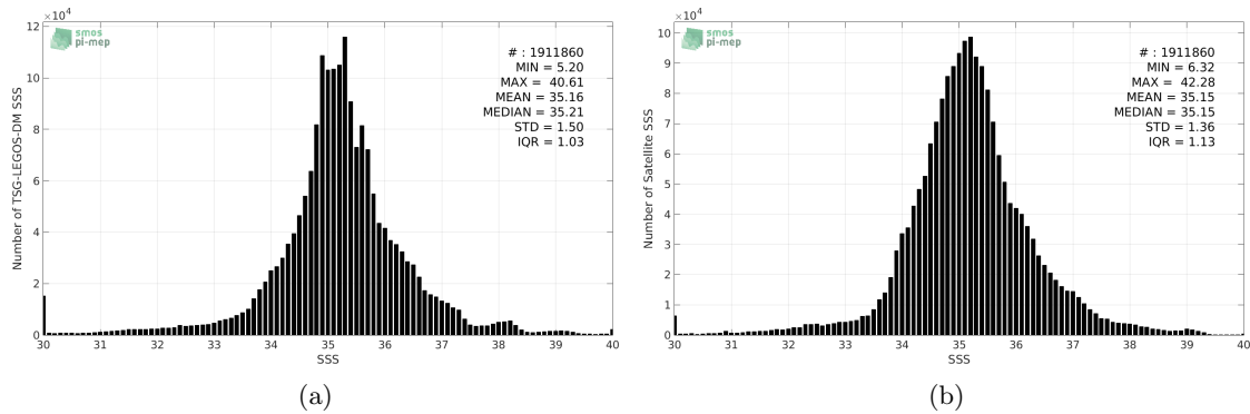
Figure 2: Histograms of SSS from TSG-LEGOS-DM (a) and SMOS-L3-CATDS-CECOS-LOCEAN-V3-18DAYS-25KM (b) considering all match-up pairs per bins of 0.1 over the SMOS coastal zone ( \leq 800 km) 60N-60S Pi-MEP region and for the full satellite product period.
