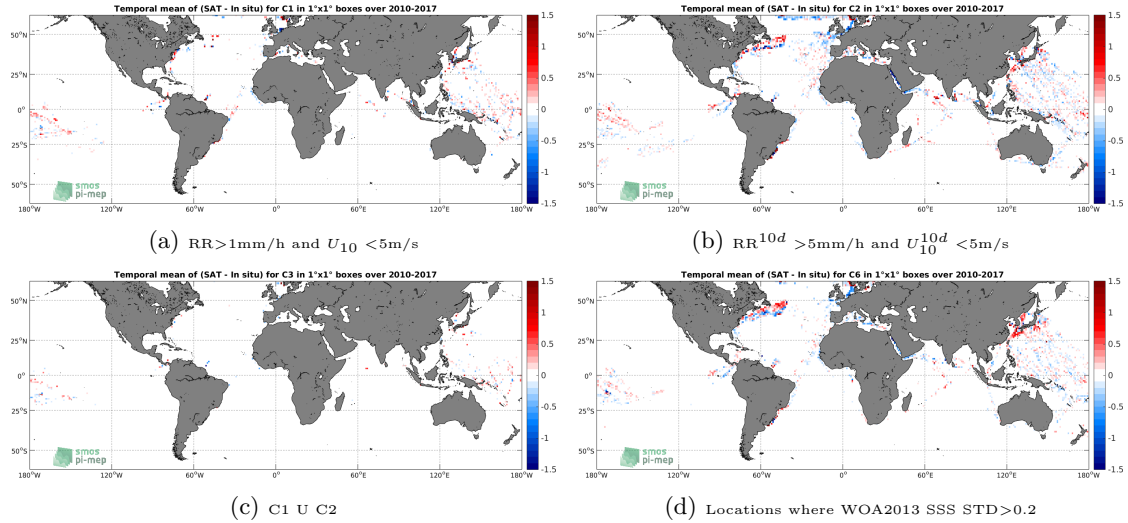
Figure 12: Temporal mean gridded over spatial boxes of size 1^\circ \times 1^\circ of \Delta SSS (SMOS-L3-CATDS-CECOS-LOCEAN-V3-18DAYS-25KM - TSG-LEGOS-DM) for 4 different subdatasets corresponding to: RR > 1\text{mm/h} and U_{10} < 5\text{m/s} (a), RR^{10d} > 5\text{mm/h} and U_{10}^{10d} < 5\text{m/s} (b), C1 U C2 (c), Locations where WOA2013 SSS STD > 0.2 (d).
