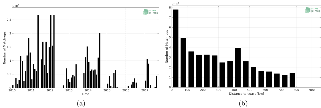
Figure 1: Number of match-ups between TSG-GOSUD-Sailing-ship and SMOS-L3-CATDS-CECOS-LOCEAN-V3-18DAYS-25KM SSS as a function of time (a) and as function of the distance to coast (b) over the SMOS coastal zone ( \approx 800 km) 60N-60S Pi-MEP region and for the full satellite product period.
