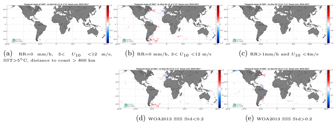
Figure 12: Temporal mean gridded over spatial boxes of size 1^\circ \times 1^\circ of \Delta\text{SSS} (SMOS-L3-CATDS-CECOS-LOCEAN-V3-18DAYS-25KM - TSG-GOSUD-Sailing-ship) for 5 different subdatasets corresponding to:RR=0 mm/h, 3 < U_{10} < 12 m/s, SST>5°C, distance to coast > 800 km (a), RR=0 mm/h, 3 < U_{10} < 12 m/s (b), RR>1mm/h and U_{10} < 4 m/s (c), WOA2013 SSS Std<0.2 (d), WOA2013 SSS Std>0.2 (e).
