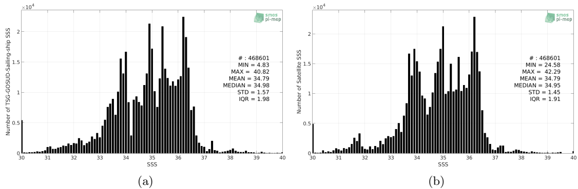
Figure 2: Histograms of SSS from TSG-GOSUD-Sailing-ship (a) and SMOS-L3-CATDS-CECOS-LOCEAN-V3-18DAYS-25KM (b) considering all match-up pairs per bins of 0.1 over the SMOS coastal zone ( \approx 800 km) 60N-60S Pi-MEP region and for the full satellite product period.
