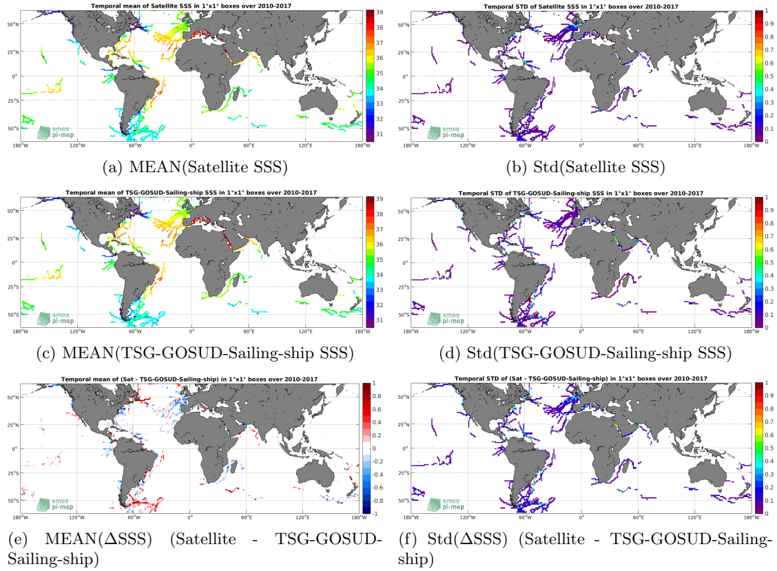
Figure 6: Temporal mean (left) and Std (right) of SSS from SMOS-L3-CATDS-CECOS-LOCEAN-V3-18DAYS-25KM (top), TSG-GOSUD-Sailing-ship (middle), and of \Delta SSS (Satellite - TSG-GOSUD-Sailing-ship). Only match-up pairs are used to generate these maps.
