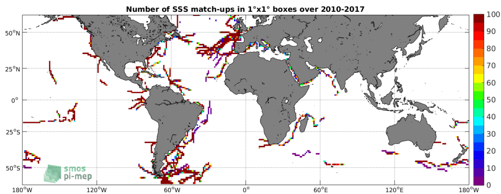
Figure 4: Number of SSS match-ups between TSG-GOSUD-Sailing-ship SSS and the SMOS-L3-CATDS-CECOS-LOCEAN-V3-18DAYS-25KM SSS product for the SMOS coastal zone ( \pm 800 km) 60N-60S Pi-MEP region over 1^\circ \times 1^\circ boxes and for the full satellite product period.
