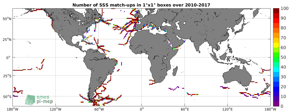
Figure 4: Number of SSS match-ups between TSG-GOSUD-Sailing-ship SSS and the SMOS-L3-CATDS-CECOS-LOCEAN-V3-18DAYS-25KM SSS product for the SMOS coastal zone ( \pm 800\text{km} ) 60N-60S Pi-MEP region over 1^\circ \times 1^\circ boxes and for the full satellite product period.
