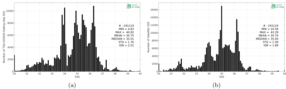
Figure 2: Histograms of SSS from TSG-GOSUD-Sailing-ship (a) and SMOS-L3-CATDS-CECOS-LOCEAN-V3-18DAYS-25KM (b) considering all match-up pairs per bins of 0.1 over the SMOS coastal zone ( \approx 800 km) 60N-60S Pi-MEP region and for the full satellite product period.
