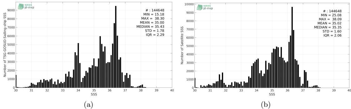
Figure 2: Histograms of SSS from TSG-GOSUD-Sailing-ship (a) and SMOS-L3-CATDS-CECOS-LOCEAN-V3-18DAYS-25KM (b) considering all match-up pairs per bins of 0.1 over the SMOS coastal zone ( \pm 800 km) 60N-60S Pi-MEP region and for the full satellite product period.
