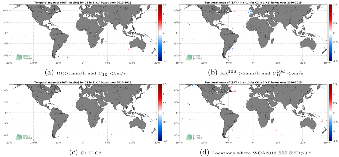
Figure 12: Temporal mean gridded over spatial boxes of size 1^\circ \times 1^\circ of \Delta SSS (SMOS-L3-CATDS-CECOS-LOCEAN-V3-18DAYS-25KM - TSG-GOSUD-Sailing-ship) for 4 different subdatasets corresponding to: RR > 1\text{mm/h} and U_{10} < 5\text{m/s} (a), RR^{10d} > 5\text{mm/h} and U_{10}^{10d} < 5\text{m/s} (b), C1 U C2 (c), Locations where WOA2013 SSS STD > 0.2 (d).
