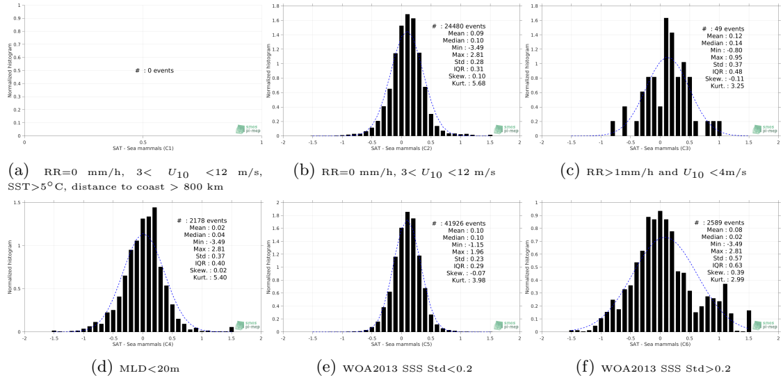
Figure 13: Normalized histogram of \Delta\text{SSS} (SMOS-L3-CATDS-CECOS-LOCEAN-V3-18DAYS-25KM - Sea mammals) for 6 different subdatasets corresponding to: RR=0 mm/h, 3 < U_{10} < 12 m/s, SST > 5^\circ\text{C} , distance to coast > 800 km (a), RR=0 mm/h, 3 < U_{10} < 12 m/s (b), RR > 1 mm/h and U_{10} < 4 m/s (c), MLD < 20 m (d), WOA2013 SSS Std < 0.2 (e), WOA2013 SSS Std > 0.2 (f).
