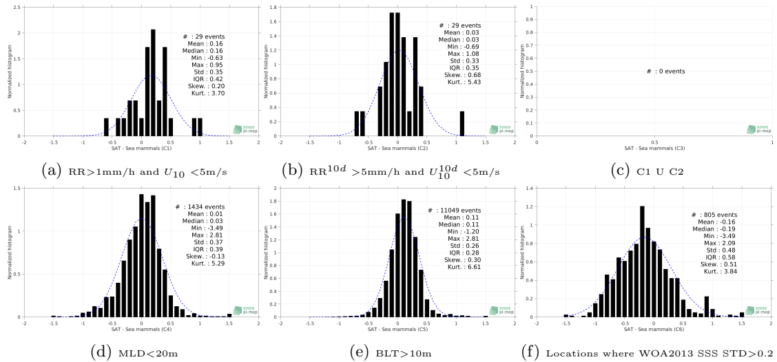
Figure 13: Normalized histogram of \Delta SSS (SMOS-L3-CATDS-CECOS-LOCEAN-V3-18DAYS-25KM - Sea mammals) for 6 different subdatasets corresponding to: RR > 1\text{mm/h} and U_{10} < 5\text{m/s} (a), RR^{10d} > 5\text{mm/h} and U_{10}^{10d} < 5\text{m/s} (b), C1 U C2 (c), MLD < 20\text{m} (d), BLT > 10\text{m} (e), Locations where WOA2013 SSS STD > 0.2 (f).
