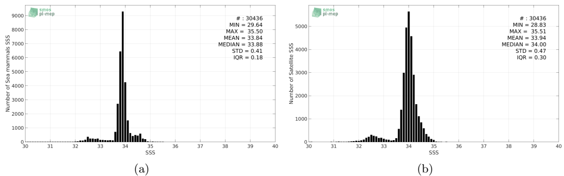
Figure 2: Histograms of SSS from Sea mammals (a) and SMOS-L3-CATDS-CECOS-LOCEAN-V3-18DAYS-25KM (b) considering all match-up pairs per bins of 0.1 over the SMOS coastal zone ( \geq 800 km) 60N-60S Pi-MEP region and for the full satellite product period.
