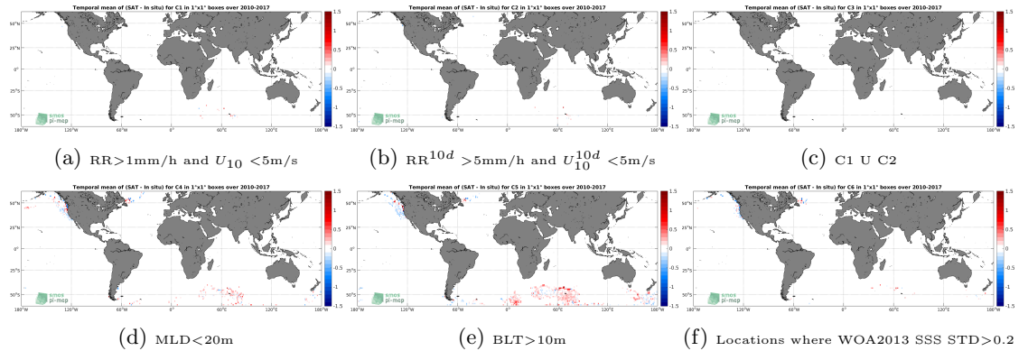
Figure 12: Temporal mean gridded over spatial boxes of size 1^\circ \times 1^\circ of \Delta SSS (SMOS-L3-CATDS-CECOS-LOCEAN-V3-18DAYS-25KM - Sea mammals) for 6 different subdatasets corresponding to: RR > 1\text{mm/h} and U_{10} < 5\text{m/s} (a), RR^{10d} > 5\text{mm/h} and U_{10}^{10d} < 5\text{m/s} (b), C1 U C2 (c), MLD < 20\text{m} (d), BLT > 10\text{m} (e), Locations where WOA2013 SSS STD > 0.2 (f).
