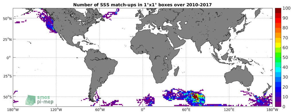
Figure 4: Number of SSS match-ups between Sea mammals SSS and the SMOS-L3-CATDS-CECOS-LOCEAN-V3-18DAYS-25KM SSS product for the SMOS coastal zone ( \approx 800\text{km} ) 60N-60S Pi-MEP region over 1^\circ \times 1^\circ boxes and for the full satellite product period.
