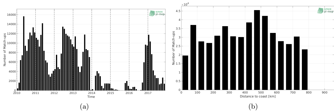
Figure 1: Number of match-ups between Surface drifters and SMOS-L3-CATDS-CECOS-LOCEAN-V3-18DAYS-25KM SSS as a function of time (a) and as function of the distance to coast (b) over the SMOS coastal zone ( \approx 800 km) 60N-60S Pi-MEP region and for the full satellite product period.
