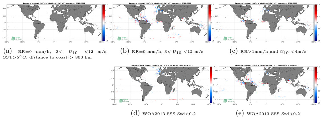
Figure 11: Temporal mean gridded over spatial boxes of size 1^\circ \times 1^\circ of \Delta SSS (SMOS-L3-CATDS-CECOS-LOCEAN-V3-18DAYS-25KM - Surface drifters) for 5 different subdatasets corresponding to:RR=0 mm/h, 3 < U_{10} < 12 m/s, SST >5^\circ C, distance to coast > 800 km (a), RR=0 mm/h, 3 < U_{10} < 12 m/s (b), RR >1 mm/h and U_{10} < 4 m/s (c), WOA2013 SSS Std <0.2 (d), WOA2013 SSS Std >0.2 (e).
