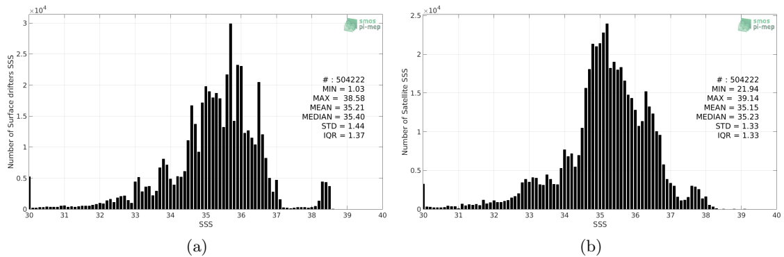
Figure 2: Histograms of SSS from Surface drifters (a) and SMOS-L3-CATDS-CECOS-LOCEAN-V3-18DAYS-25KM (b) considering all match-up pairs per bins of 0.1 over the SMOS coastal zone ( \approx 800\text{km} ) 60N-60S Pi-MEP region and for the full satellite product period.
