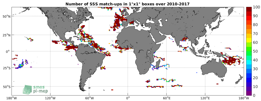
Figure 3: Number of SSS match-ups between Surface drifters SSS and the SMOS-L3-CATDS-CECOS-LOCEAN-V3-18DAYS-25KM SSS product for the SMOS coastal zone ( \approx 800\text{km} ) 60N-60S Pi-MEP region over 1^\circ \times 1^\circ boxes and for the full satellite product period.
