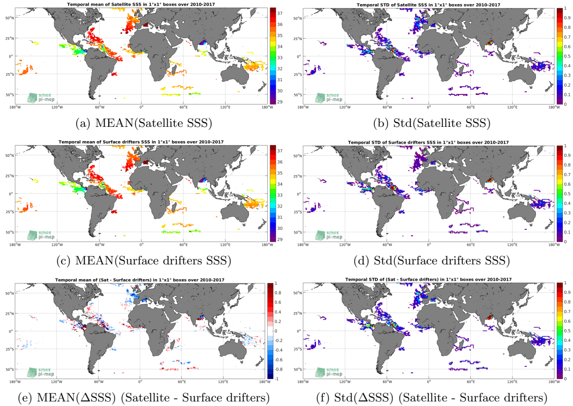
Figure 5: Temporal mean (left) and Std (right) of SSS from SMOS-L3-CATDS-CECOS-LOCEAN-V3-18DAYS-25KM (top), Surface drifters (middle), and of \Delta SSS (Satellite - Surface drifters). Only match-up pairs are used to generate these maps.
