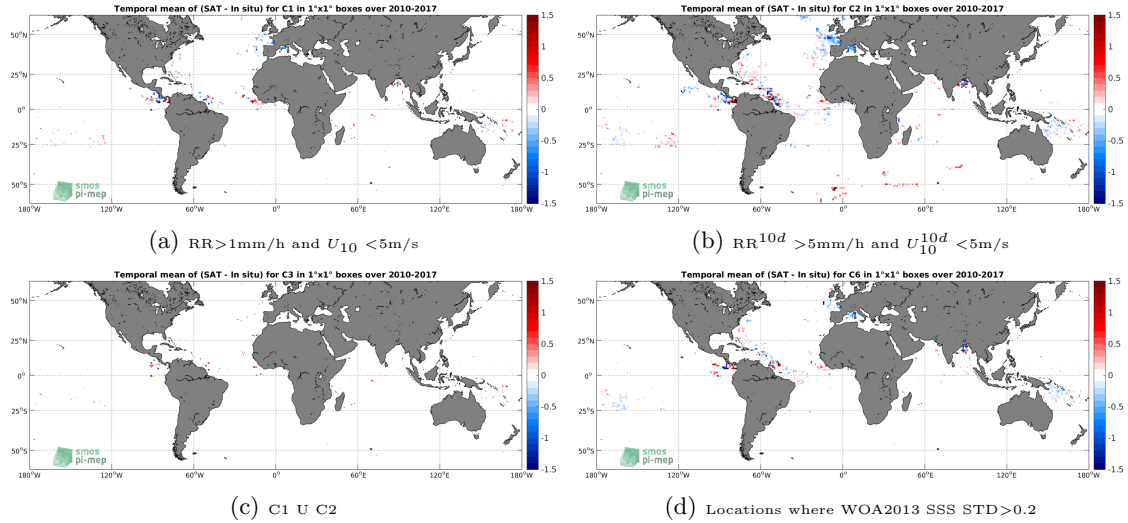
Figure 11: Temporal mean gridded over spatial boxes of size 1^\circ \times 1^\circ of \Delta SSS (SMOS-L3-CATDS-CECOS-LOCEAN-V3-18DAYS-25KM - Surface drifters) for 4 different subdatasets corresponding to: RR > 1\text{mm/h} and U_{10} < 5\text{m/s} (a), RR^{10d} > 5\text{mm/h} and U_{10}^{10d} < 5\text{m/s} (b), C1 U C2 (c), Locations where WOA2013 SSS STD > 0.2 (d).
