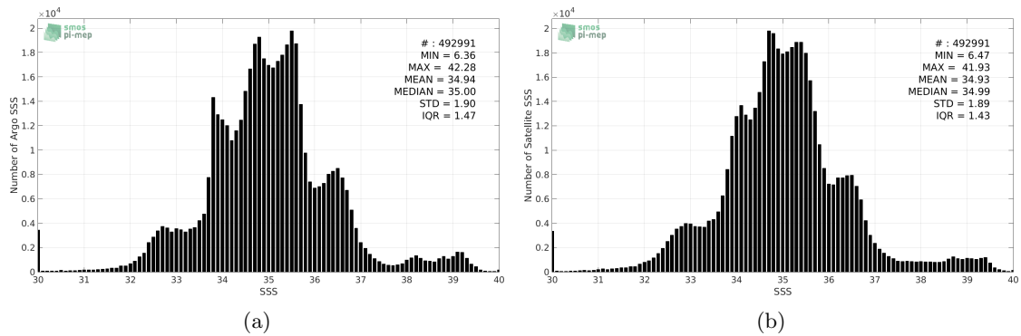
Figure 2: Histograms of SSS from Argo (a) and SMOS-L3-CATDS-CECOS-LOCEAN-V3-18DAYS-25KM (b) considering all match-up pairs per bins of 0.1 over the SMOS coastal zone ( \approx 800\text{km} ) 60N-60S Pi-MEP region and for the full satellite product period.
