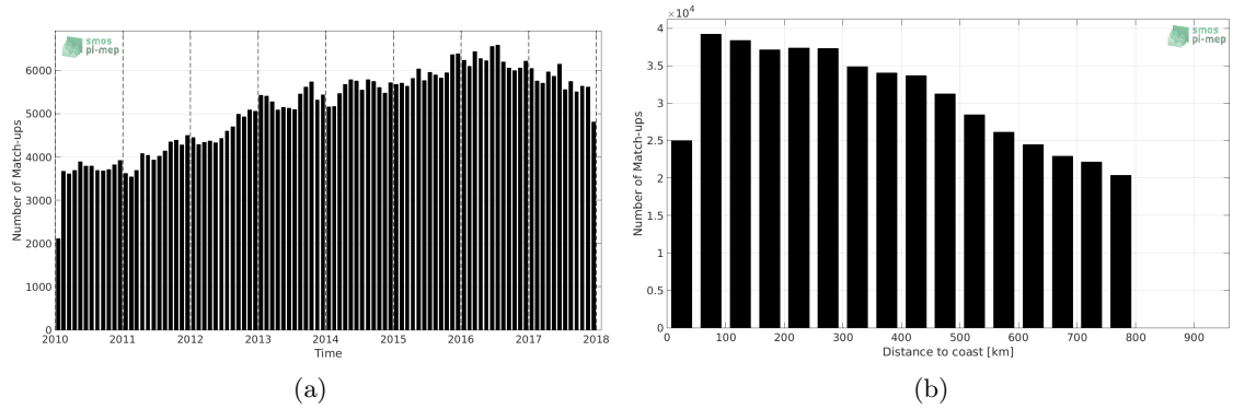
Figure 1: Number of match-ups between Argo and SMOS-L3-CATDS-CECOS-LOCEAN-V3-18DAYS-25KM SSS as a function of time (a) and as function of the distance to coast (b) over the SMOS coastal zone ( \approx 800\text{km} ) 60N-60S Pi-MEP region and for the full satellite product period.
