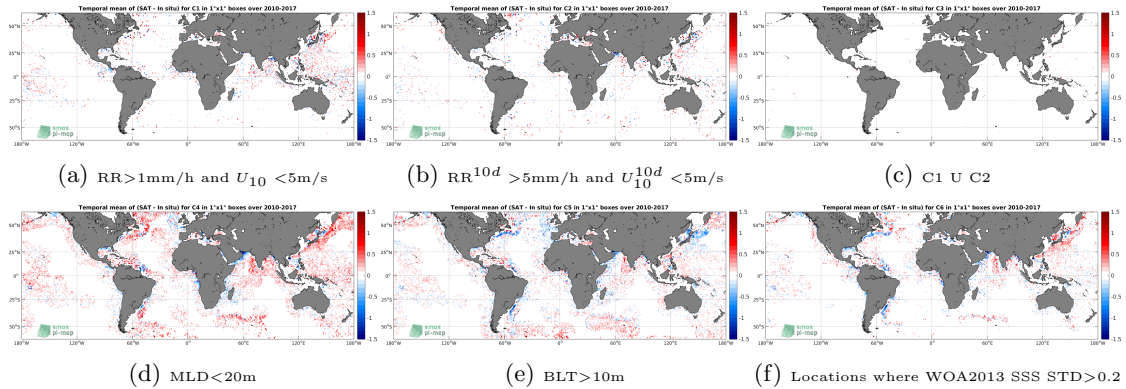
Figure 12: Temporal mean gridded over spatial boxes of size 1^\circ \times 1^\circ of \Delta SSS (SMOS-L3-CATDS-CECOS-LOCEAN-V3-18DAYS-25KM - Argo) for 6 different subdatasets corresponding to: RR > 1\text{mm/h} and U_{10} < 5\text{m/s} (a), RR^{10d} > 5\text{mm/h} and U_{10}^{10d} < 5\text{m/s} (b), C1 U C2 (c), MLD < 20\text{m} (d), BLT > 10\text{m} (e), Locations where WOA2013 SSS STD > 0.2 (f).
