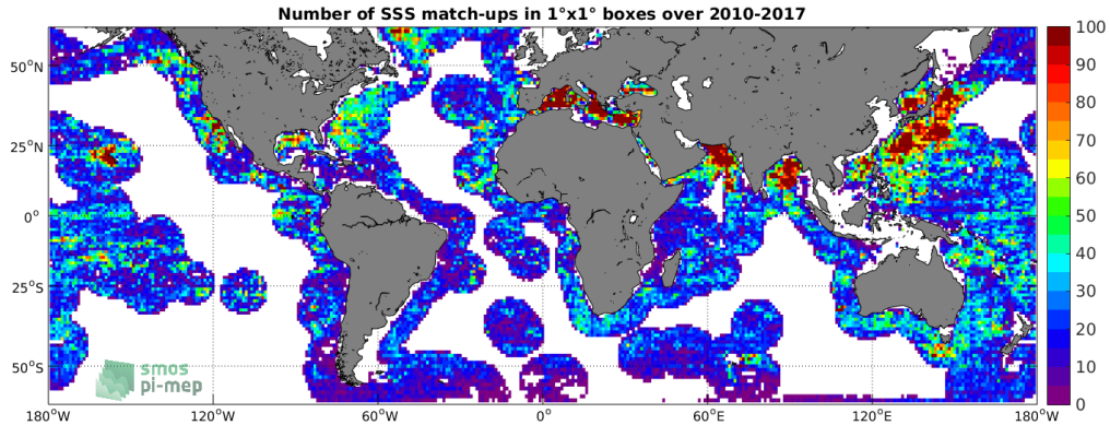
Figure 4: Number of SSS match-ups between Argo SSS and the SMOS-L3-CATDS-CECOS-LOCEAN-V3-18DAYS-25KM SSS product for the SMOS coastal zone ( \approx 800\text{km} ) 60N-60S Pi-MEP region over 1^\circ \times 1^\circ boxes and for the full satellite product period.
