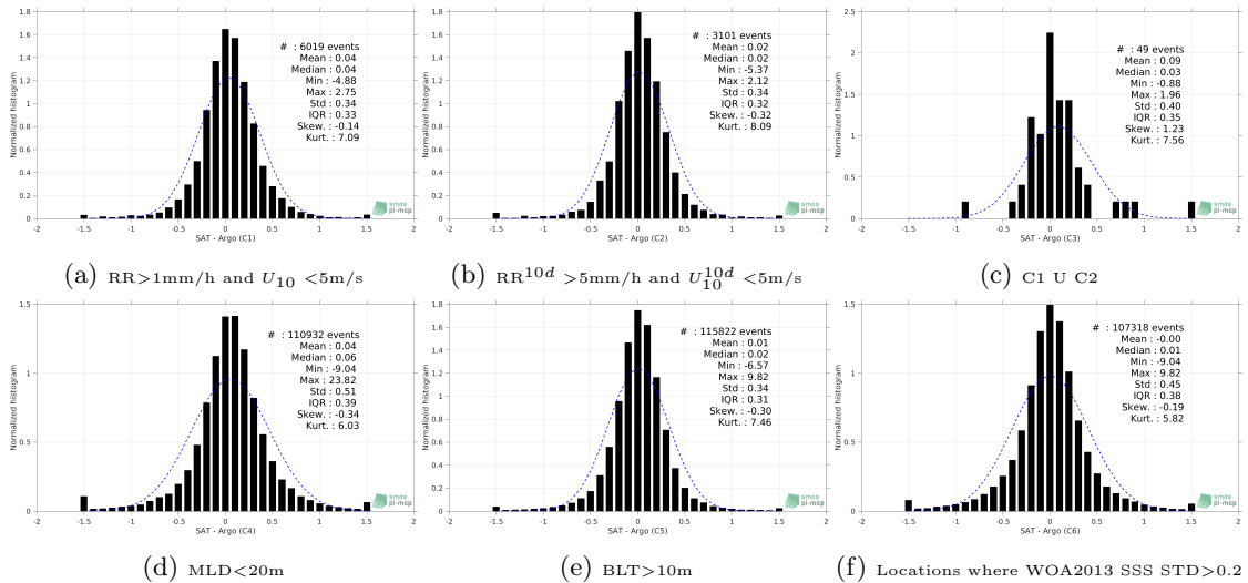
Figure 13: Normalized histogram of \Delta SSS (SMOS-L3-CATDS-CECOS-LOCEAN-V3-18DAYS-25KM - Argo) for 6 different subdatasets corresponding to: RR > 1\text{mm/h} and U_{10} < 5\text{m/s} (a), RR^{10d} > 5\text{mm/h} and U_{10}^{10d} < 5\text{m/s} (b), C1 U C2 (c), MLD < 20\text{m} (d), BLT > 10\text{m} (e), Locations where WOA2013 SSS STD > 0.2 (f).
