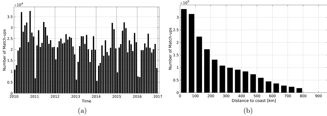
Figure 1: Number of match-ups between TSG-LEGOS-DM and SMOS-L3-CATDS-CECOS-LOCEAN-V2-9DAYS-25KM SSS as a function of time (a) and as function of the distance to coast (b) over the SMOS coastal zone ( \approx 800\text{km} ) 60N-60S Pi-MEP region and for the full satellite product period.
