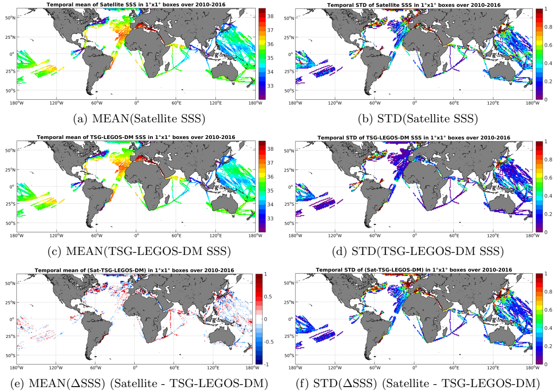
Figure 6: Temporal mean (left) and STD (right) of SSS from SMOS-L3-CATDS-CECOS-LOCEAN-V2-9DAYS-25KM (top), TSG-LEGOS-DM (middle), and of \Delta SSS (Satellite - TSG-LEGOS-DM). Only match-up pairs are used to generate these maps.
