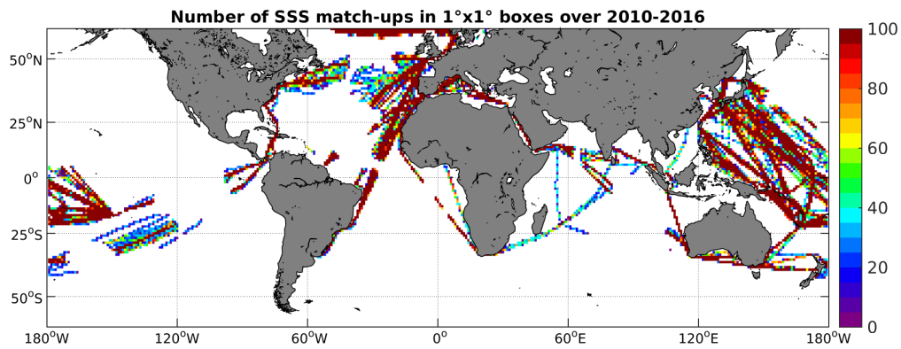
Figure 4: Number of SSS match-ups between TSG-LEGOS-DM SSS and the SMOS-L3-CATDS-CECOS-LOCEAN-V2-9DAYS-25KM SSS product for the SMOS coastal zone ( \geq 800\text{km} ) 60N-60S Pi-MEP region over 1^\circ \times 1^\circ boxes and for the full satellite product period.
