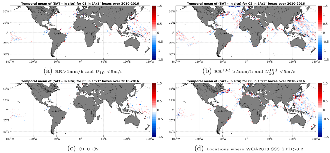
Figure 12: Temporal mean gridded over spatial boxes of size 1^\circ \times 1^\circ of \Delta SSS (SMOS-L3-CATDS-CECOS-LOCEAN-V2-9DAYS-25KM - TSG-LEGOS-DM) for 4 different subdatasets corresponding to: RR > 1\text{mm/h} and U_{10} < 5\text{m/s} (a), RR^{10d} > 5\text{mm/h} and U_{10}^{10d} < 5\text{m/s} (b), C1 U C2 (c), Locations where WOA2013 SSS STD > 0.2 (d).
