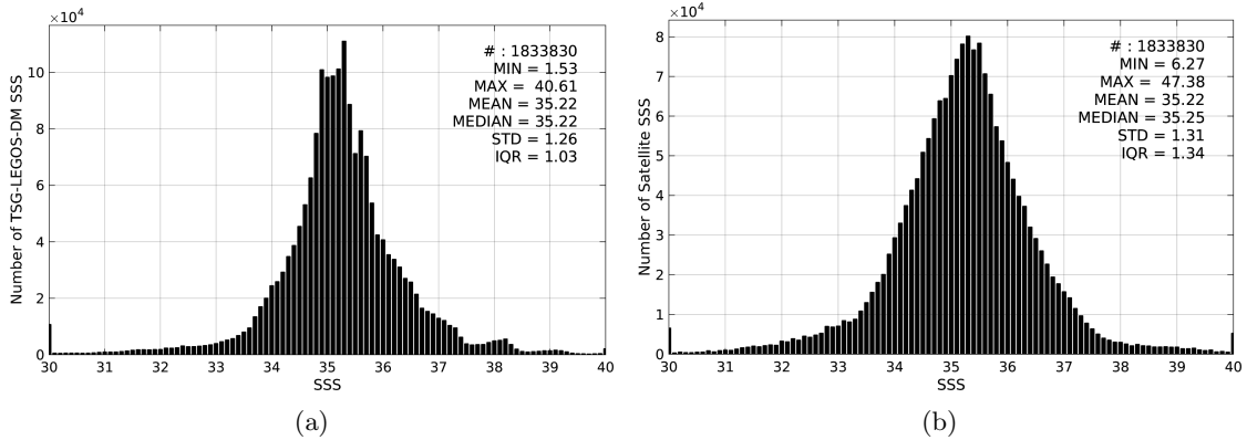
Figure 2: Histograms of SSS from TSG-LEGOS-DM (a) and SMOS-L3-CATDS-CECOS-LOCEAN-V2-9DAYS-25KM (b) considering all match-up pairs per bins of 0.1 over the SMOS coastal zone ( \approx 800\text{km} ) 60N-60S Pi-MEP region and for the full satellite product period.
