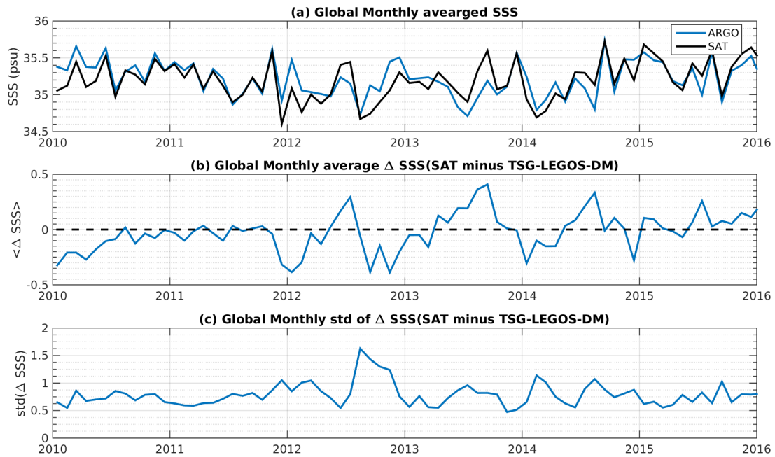
Figure 7: Time series of the monthly averaged mean SSS (top), mean \Delta SSS (Satellite - TSG-LEGOS-DM) and STD of \Delta SSS (Satellite - TSG-LEGOS-DM) over the SMOS coastal zone ( \pm 800 km) 60N-60S Pi-MEP region considering all match-ups collected by the Pi-MEP platform.
