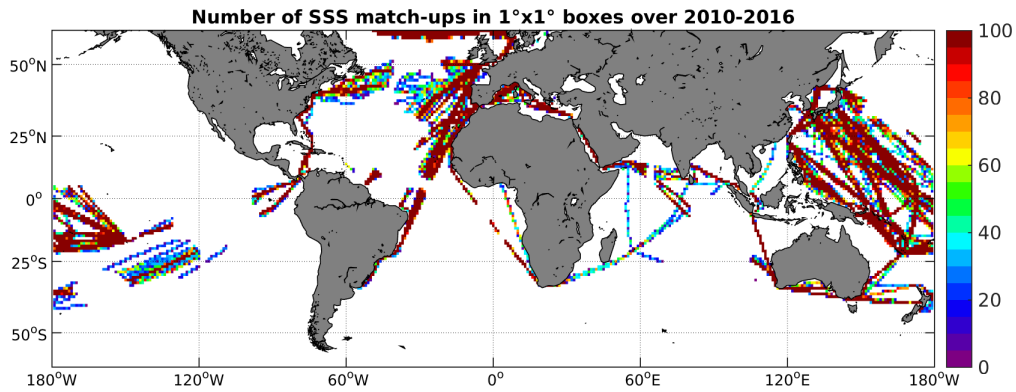
Figure 4: Number of SSS match-ups between TSG-LEGOS-DM SSS and the SMOS-L3-CATDS-CECOS-LOCEAN-V2-9DAYS-25KM SSS product for the SMOS coastal zone ( \pm 800\text{km} ) 60N-60S Pi-MEP region over 1^\circ \times 1^\circ boxes and for the full satellite product period.
